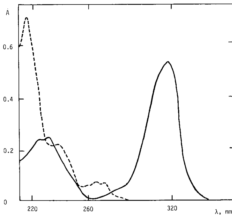
Fig 2. The uv spectrum of 10^{-5} M 2-mercaptobenzothiazole in ethanol (—); uv spectrum of the solution after photolysis (-----).
