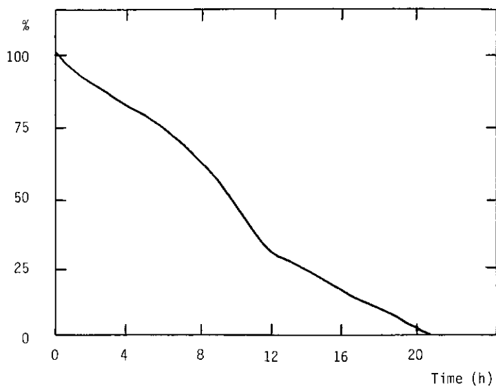
Fig. 1. Photodegradation rate of 7.7 \times 10^{-3} M solution of 2-mercaptobenzothiazole (1) in 96% ethanol (followed at 320 nm).
