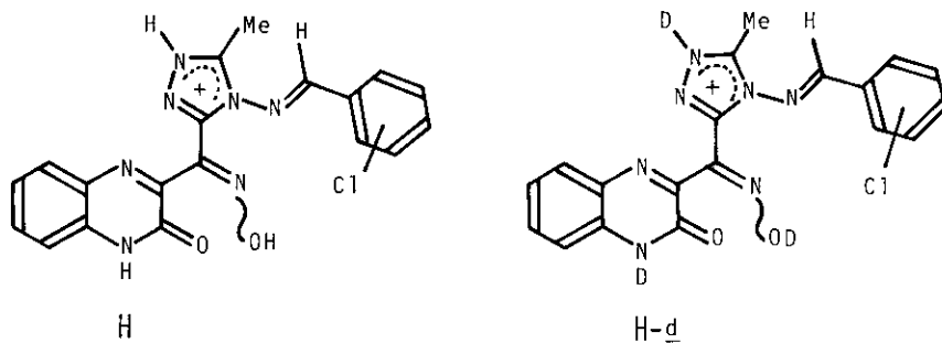
CHART 15 Species of 16c,d in TFA and TFA- \text{d}_1
