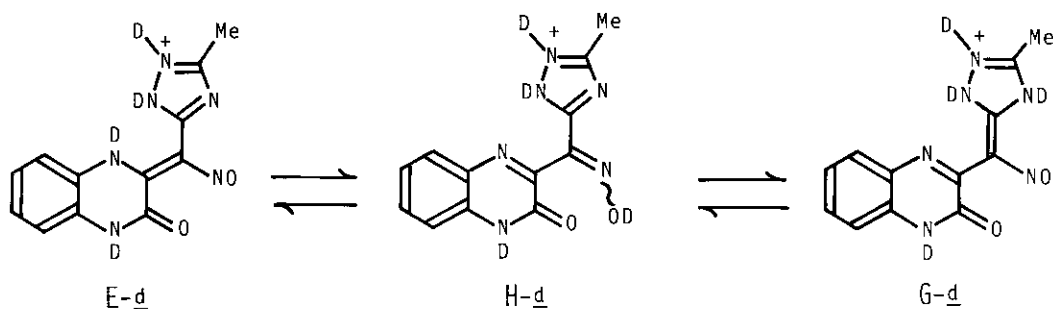
SCHEME 16 Tautomeric Equilibria of 16b in TFA- \text{d}_1 (Tautomers in Medium — Two of E-d, G-d, H-d)
