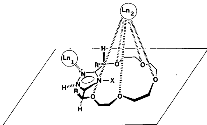
Figure 1. Complexation sites proposed for triazoly crowns 1 and 2
