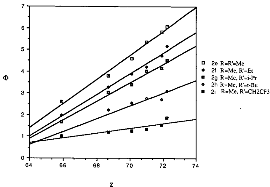
Figure 1 Relative quantum yields vs Z value
