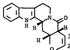
(2a) (2b); 2,3-dihydro
