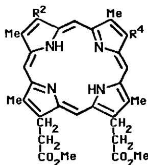
(42) R^2 = \text{H}; R^4 = \text{CH}=\text{CH}_2
