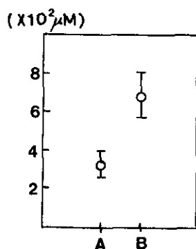
Figure 1 Graphical representation of transport of L-Phe-OMe·HCl through a liquid membrane (μM). A = cyclic octapeptide (13), B = 18-crown-6.
