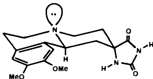
A Bucherer- Bergs product \alpha isomer
