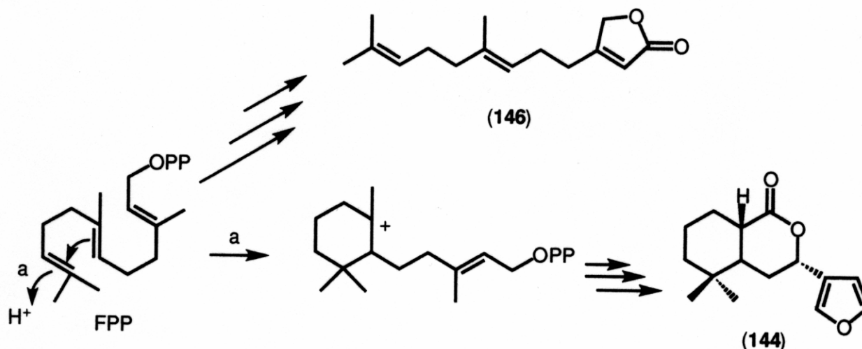
Scheme 11. Possible biogenetic pathway for monocyclofarnesenes found in Frullania and Ricciocarpus species.
