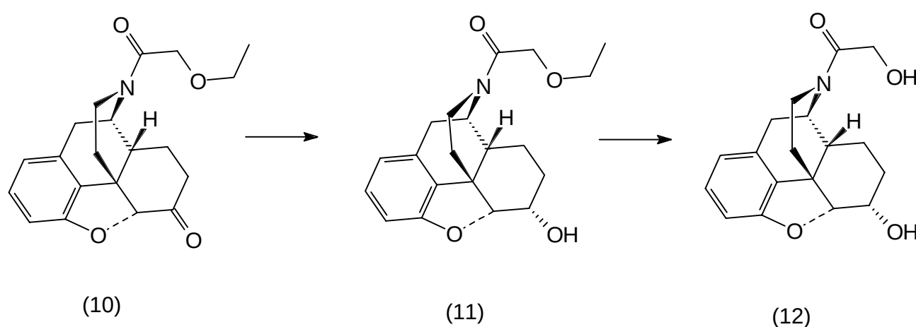
Figure 3: Microbial transformations of desoxyhydromorphinan ( 10 )
