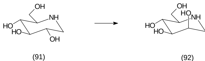
Figure 23: Microbial isomerization of 1-desoxynojirimycin
