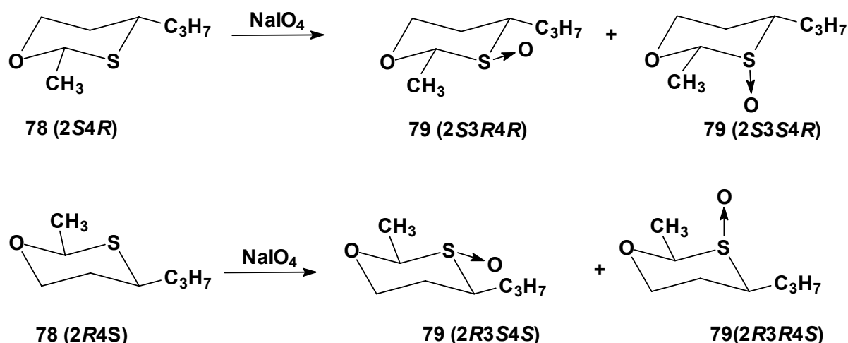
Scheme 16
