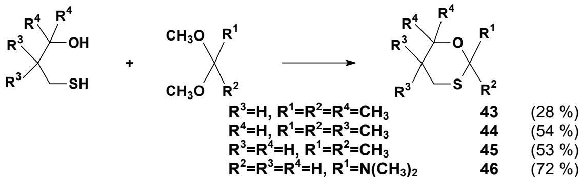
Scheme 5
