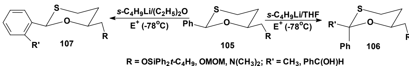
Scheme 32
