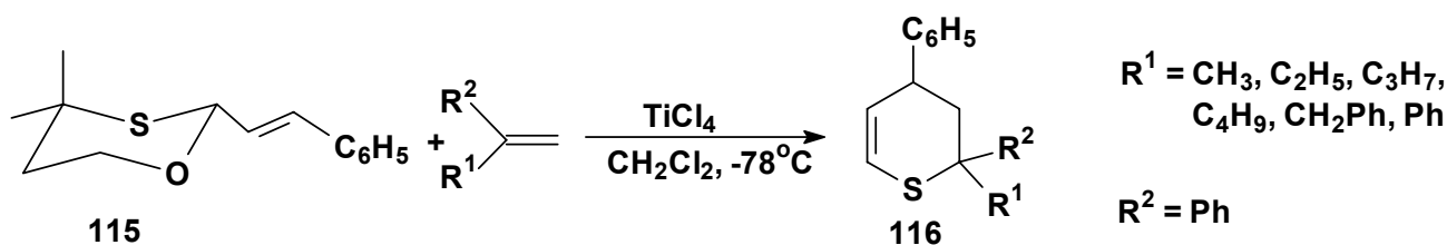
Scheme 35
