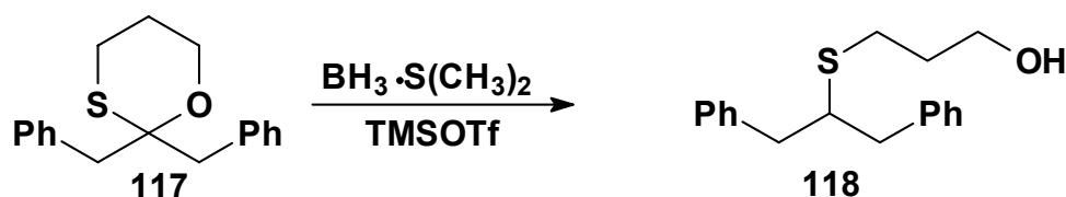
Scheme 36
