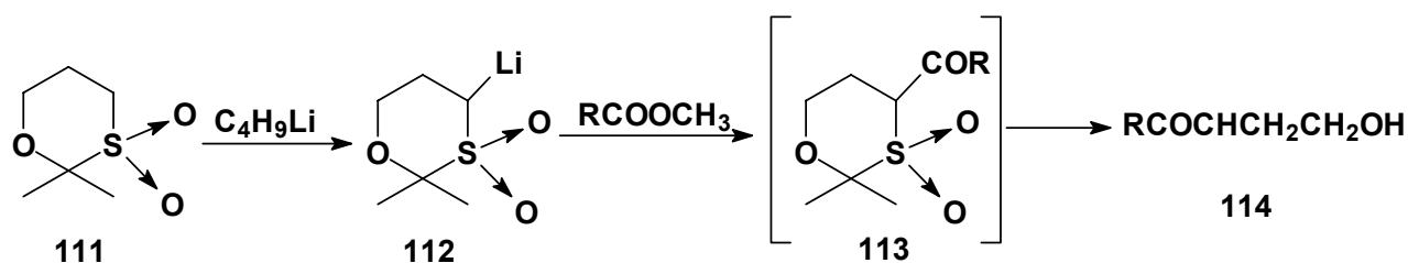
Scheme 34
