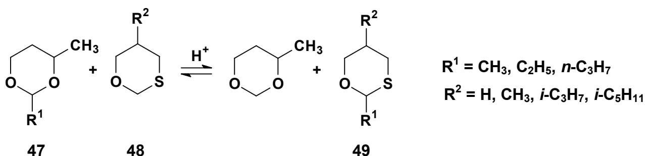
Scheme 5
