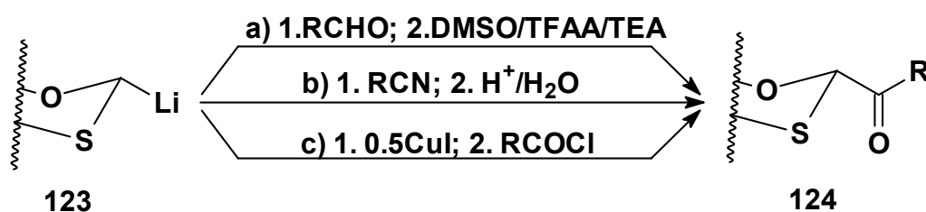
Scheme 39
