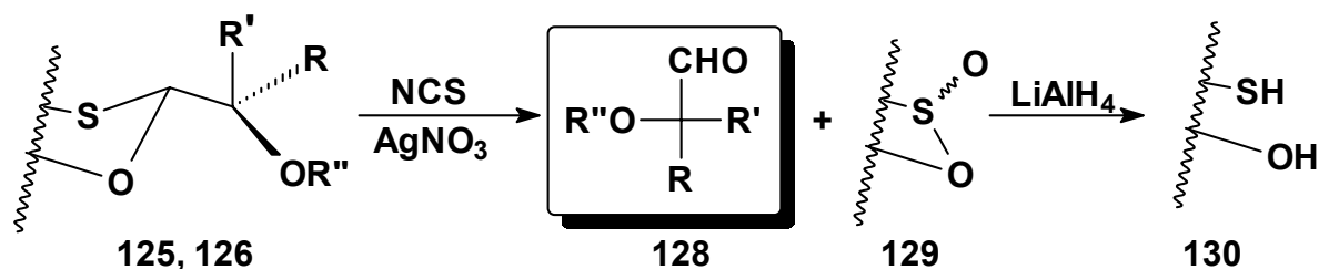
Scheme 42
