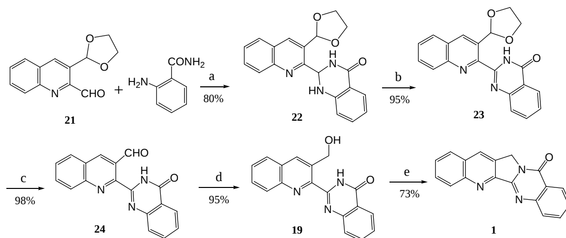
Figure 10 Reagents and conditions: a) 15% \text{NaOH} - \text{EtOH} solution, reflux, 5 h; or \text{DMA} , 80 °C, 3 h; b) \text{KMnO}_4 , acetone, reflux, 3 h; c) 10% \text{HCl} - \text{THF} , 0.5 h; d) \text{NaBH}_4 , \text{MeOH} ; e) \text{PPh}_3 , \text{DEAD} , \text{THF} ; or 60% ethanolic \text{H}_2\text{SO}_4 , reflux.
