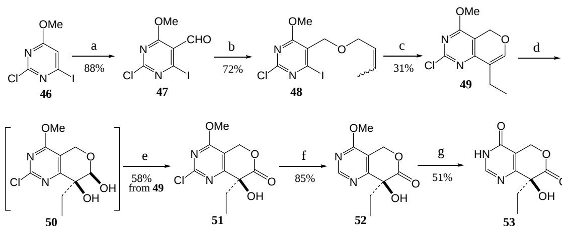
Figure 21 Reagents and conditions: a) (i) tetramethylpiperidine, n -BuLi, THF, -70 °C; (ii) HCOOEt, THF, -70 °C; (iii) aq. HCl, EtOH, THF; b) MeCH=CHCH 2 OH, TFA, Et 3 SiH, 25 °C, 16 h; c) Pd(OAc)_2 , n -Bu 4 NBr, K_2CO_3 , DMF, 85 °C, 12 h; d) (DHQD) 2 -Pyr, K_3Fe(CN)_6 , K_2CO_3 , K_2OsO_4 \cdot 2H_2O , MeSO 2 NH 2 , t -BuOH-H 2 O; e) I_2 , CaCO 3 ; f) H 2 , Pd/C, EtOH, Et 3 N, 24 h; g) 6N HCl, MeOH, reflux, 3 h.
