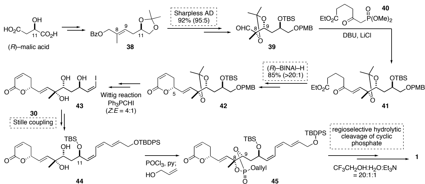
Scheme 4 Imanishi's Synthesis
