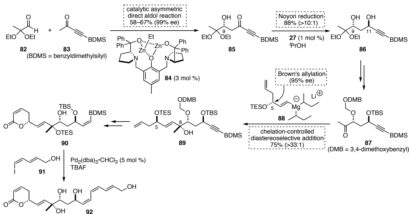
Scheme 8 Trost's Synthesis
