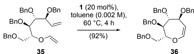
Scheme 8. Oxepine formation by RCM.
