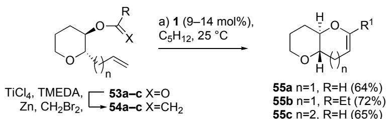
Scheme 14. Carbonyl-olefination followed by catalytic enol ether-olefin RCM as a route to fused polyethers.
