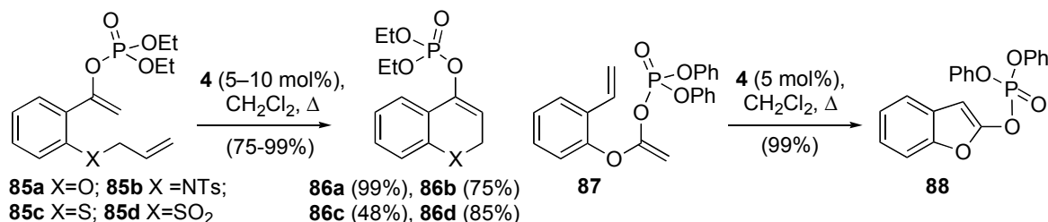
Scheme 24. RCM to afford cyclic enol phosphates.
