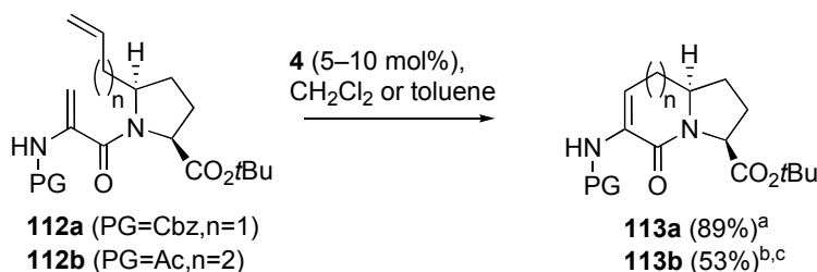
Scheme 33. RCM to give exocyclic enamides. a CH 2 Cl 2 (0.04 M), 20 °C, 5 h; b toluene (0.004 M), 100 °C, 72 h; c Some of the six membered product ( n =1, 14%) was observed.
