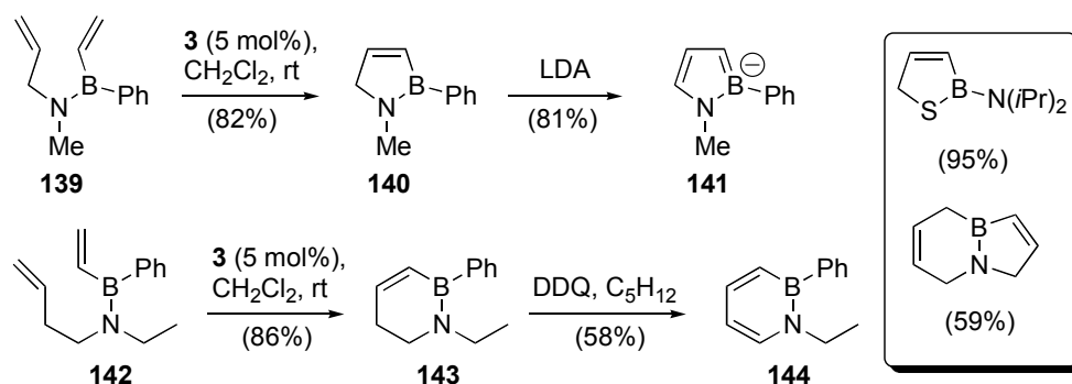
Scheme 46. Synthesis of boron-containing heterocycles.
