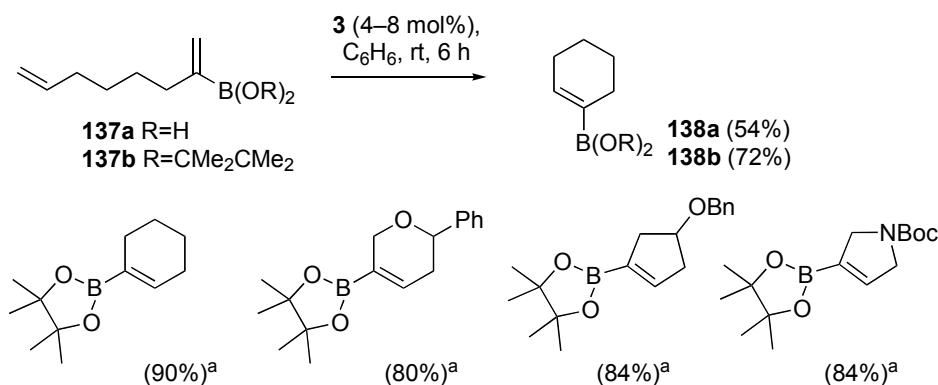
Scheme 45. Alkenylboronate–olefin RCM. a 3 (5–10 mol%) in \text{C}_6\text{H}_6 (0.004–0.05 M), rt.
