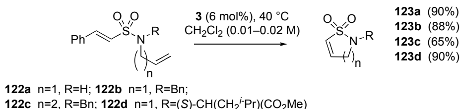
Scheme 36. RCM of vinylsulfamides.
