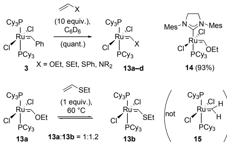
Scheme 3. Reactions of electron-rich olefins with ruthenium alkylidenes to give Fischer carbenes.
