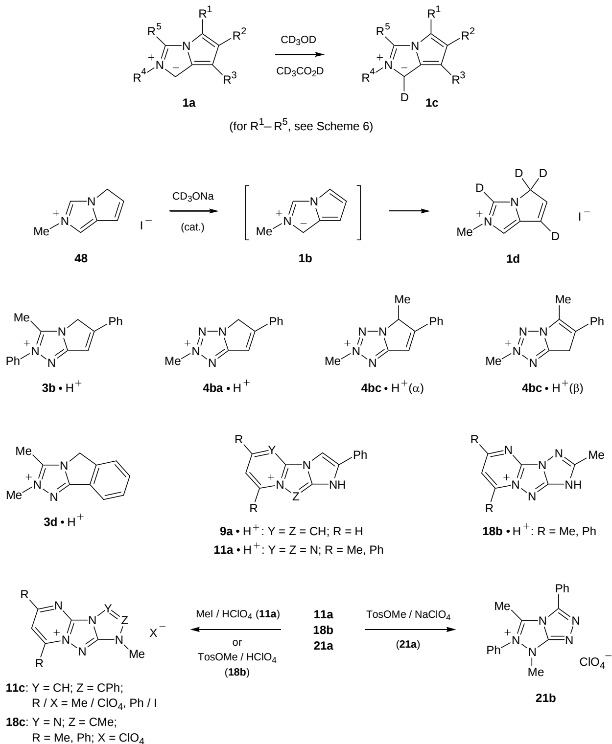
Scheme 14
