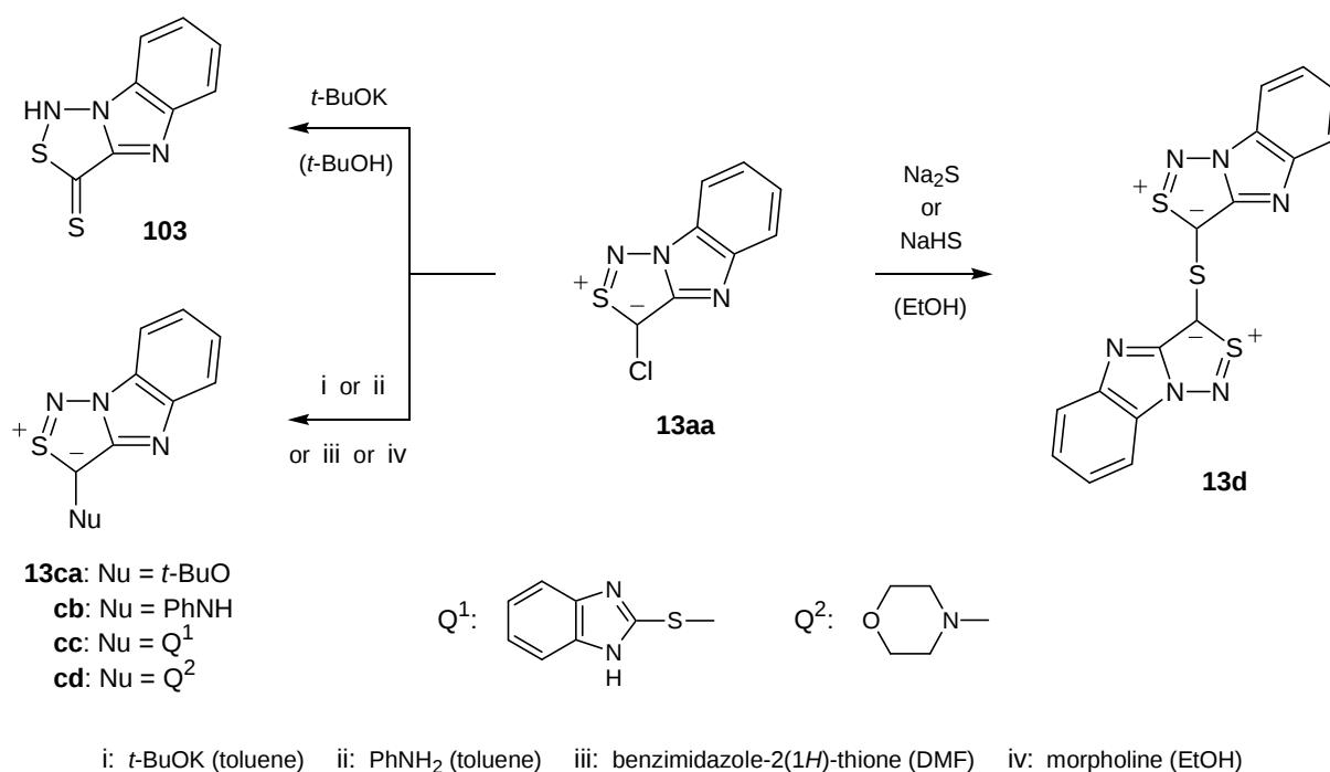
Scheme 19
