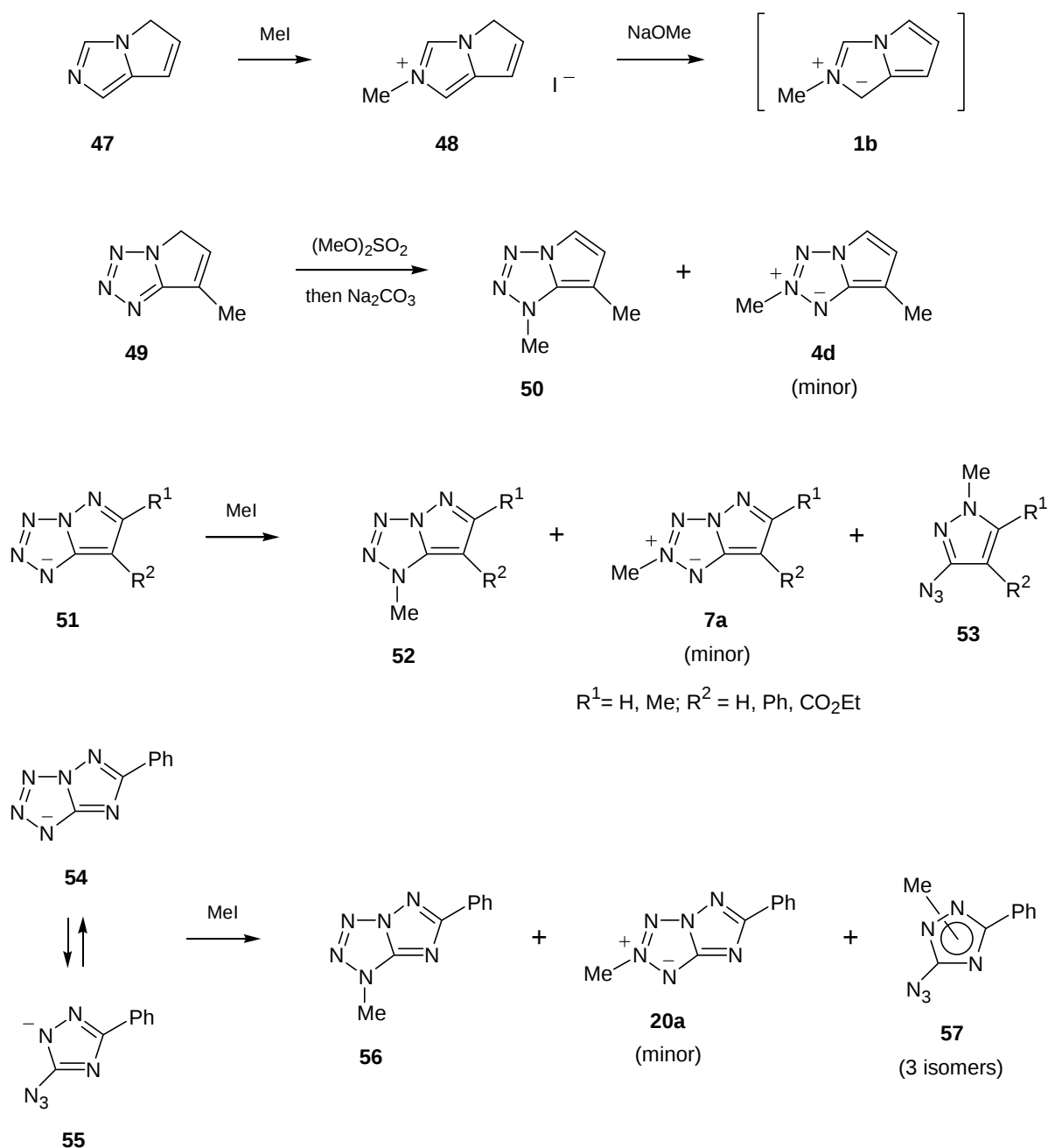
Scheme 7
