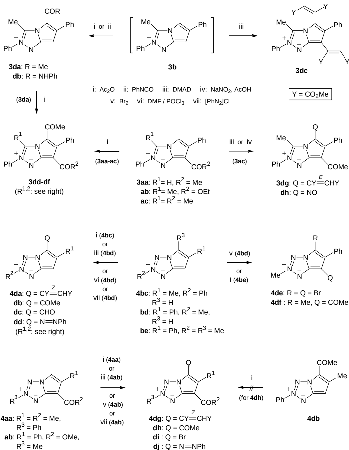
Scheme 15
