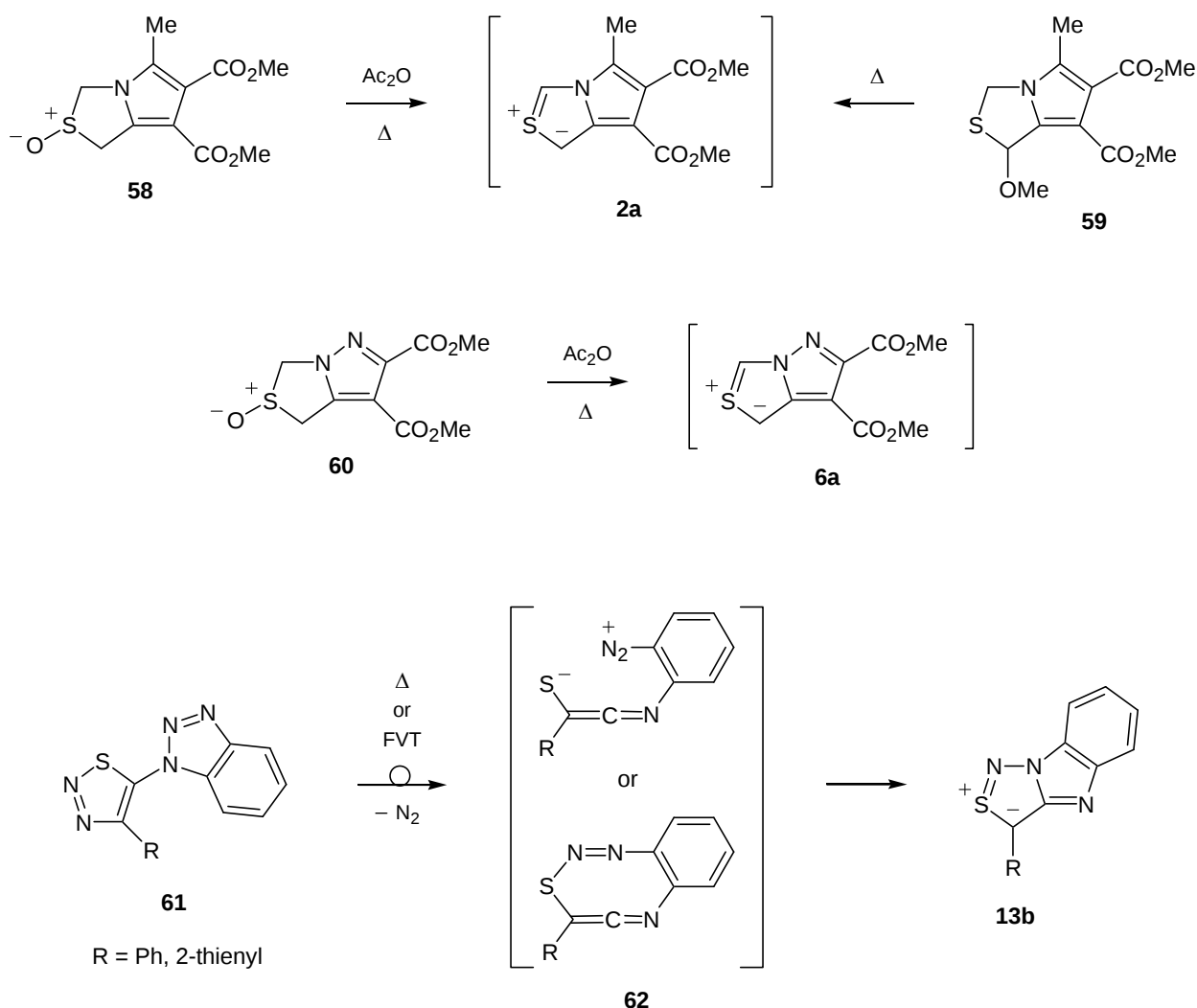
Scheme 8
