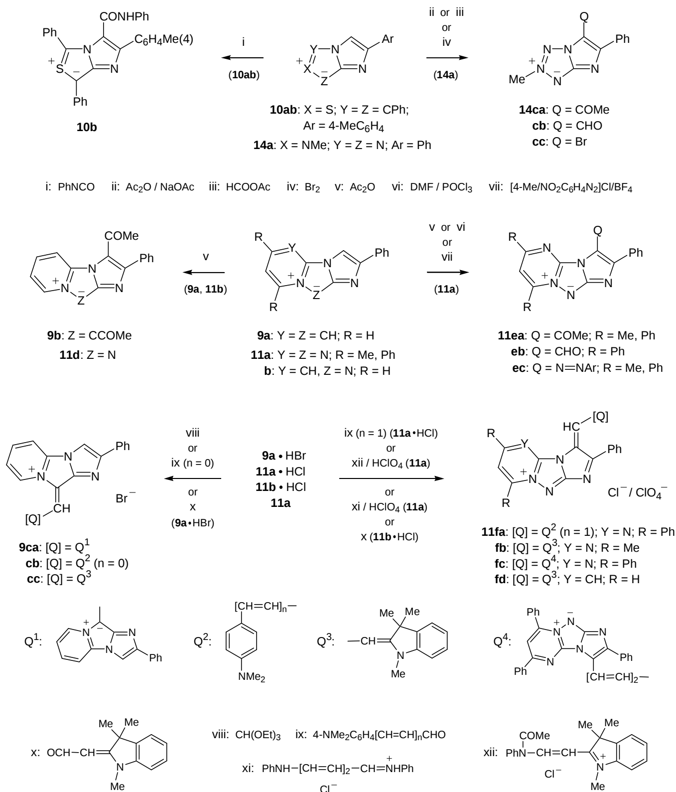
Scheme 16
