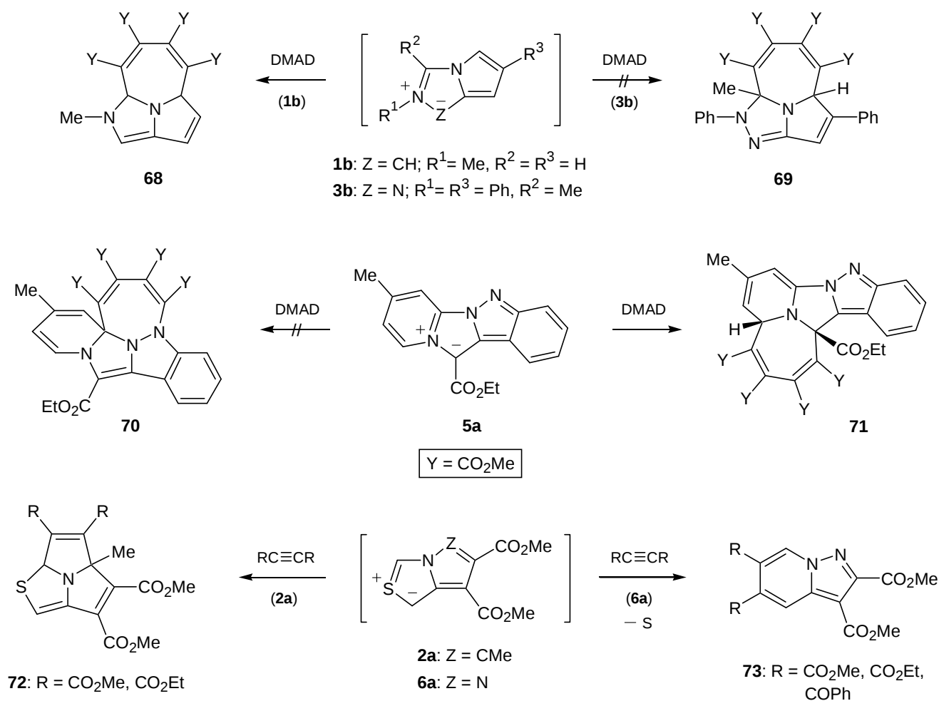
Scheme 10
