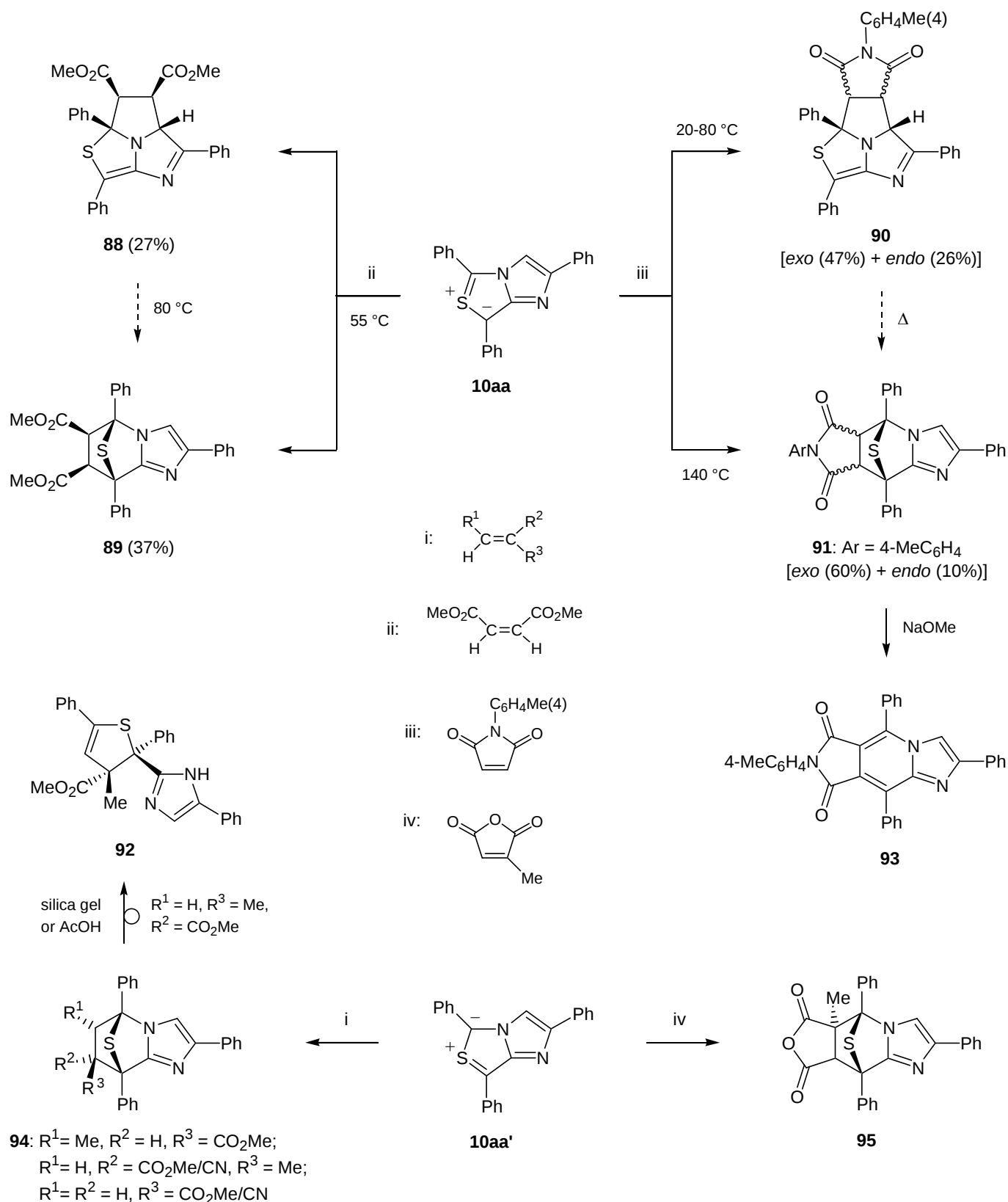
Scheme 13
