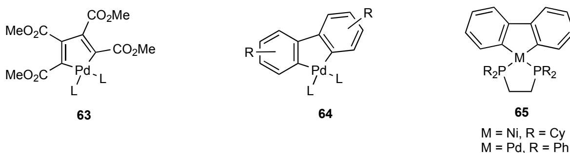
Scheme 18
