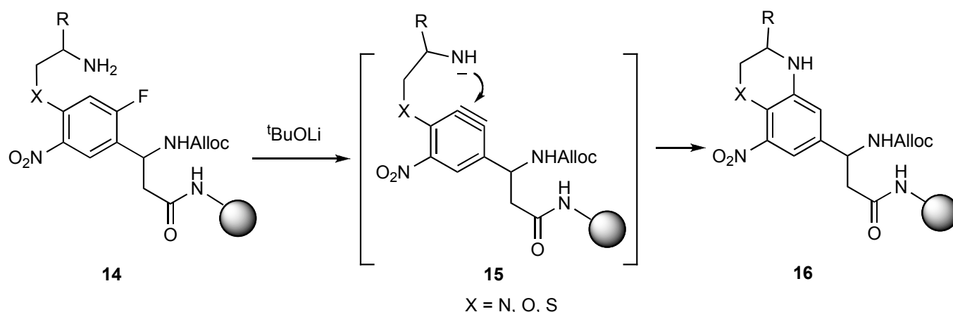
Scheme 5
