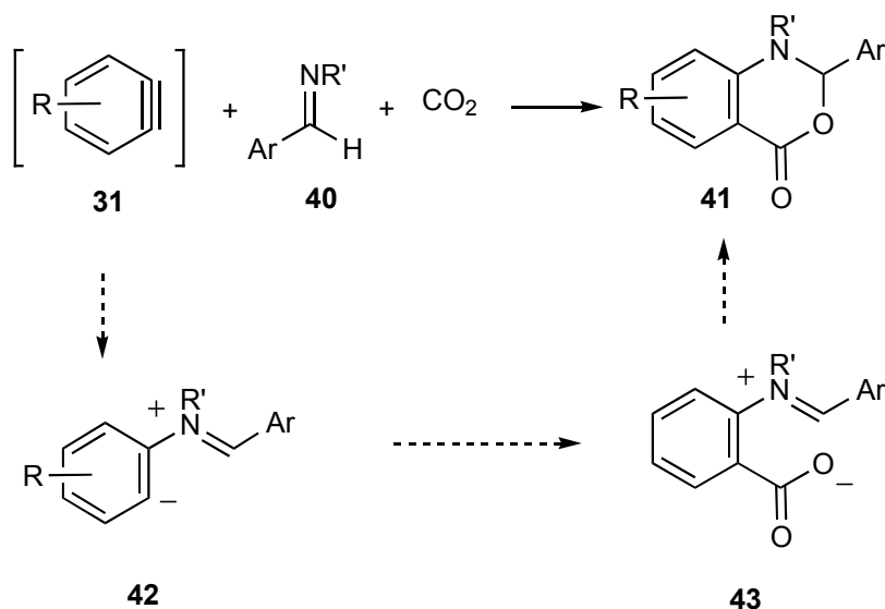
Scheme 12
