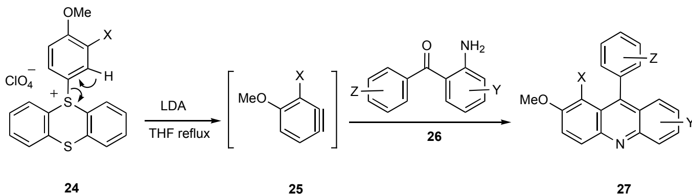
Scheme 8
