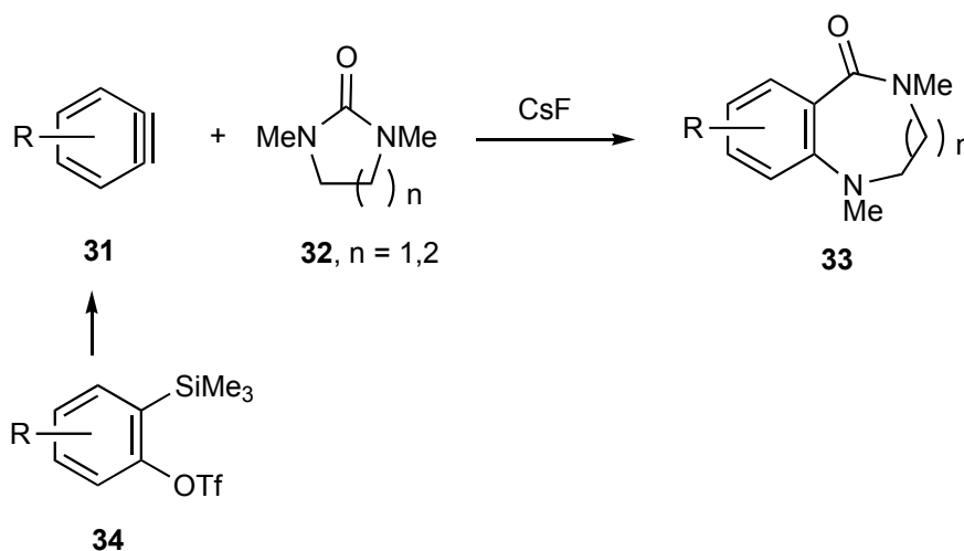
Scheme 10
