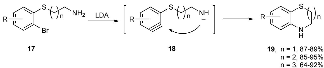
Scheme 6
