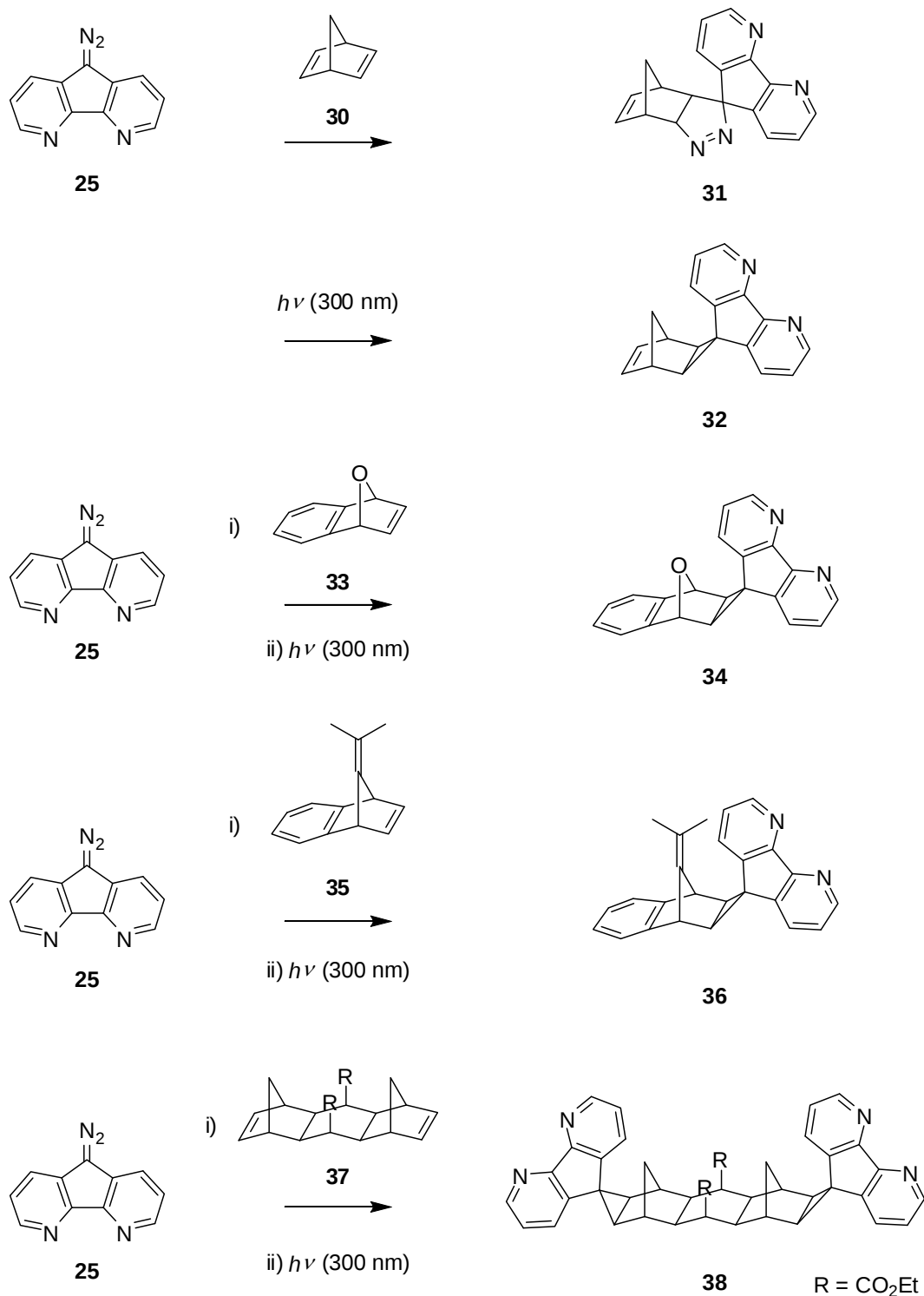
Scheme 9. Reactions of 25 with bicyclic olefins.
