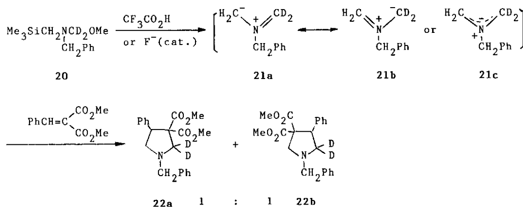
Scheme 9
