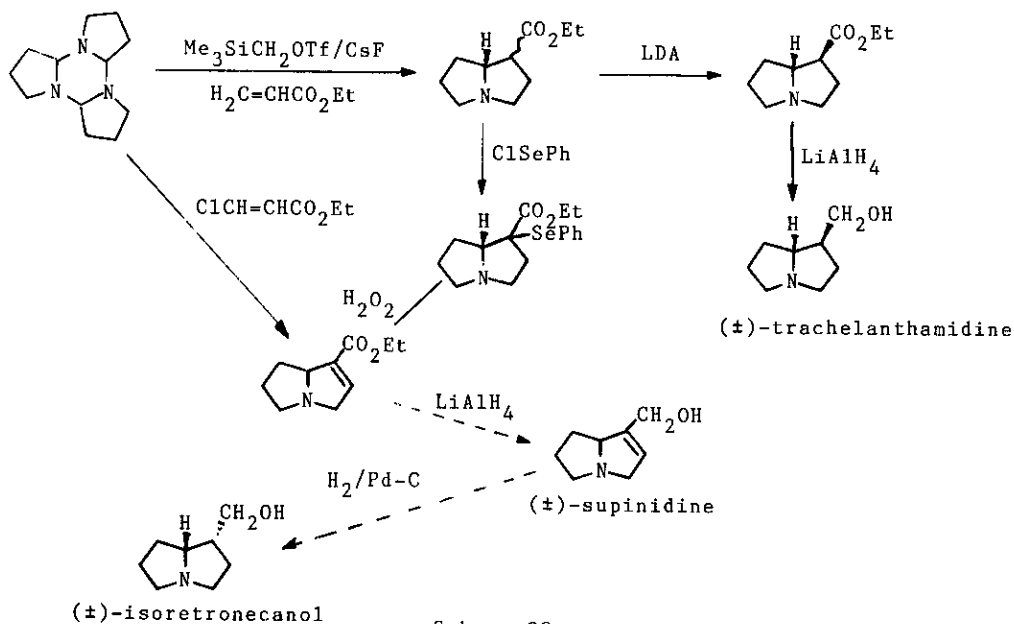
Scheme 20
