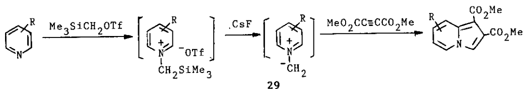
Scheme 12
