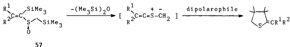
Scheme 27
