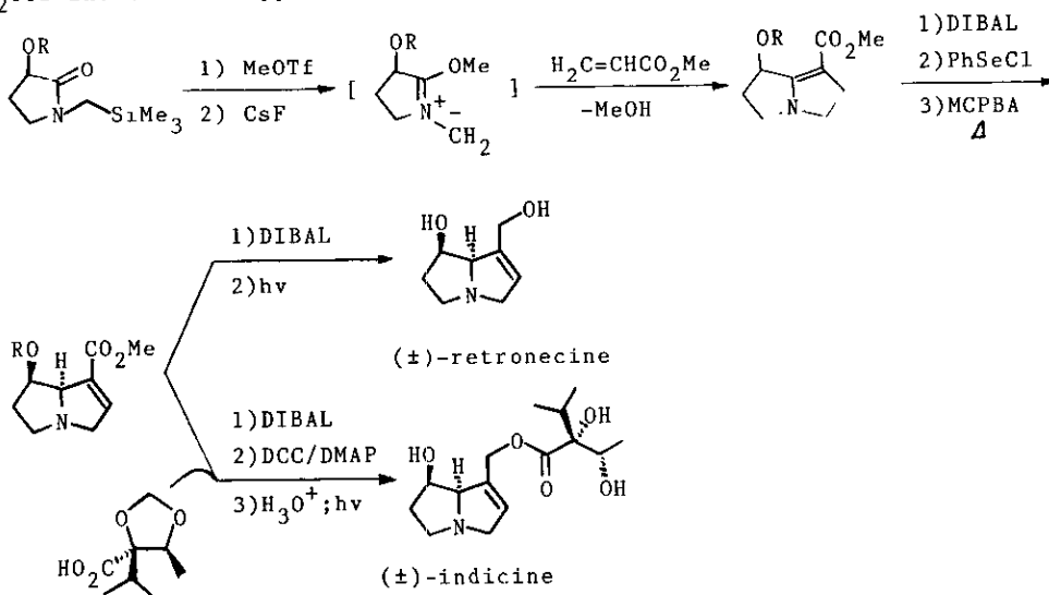
Scheme 16
