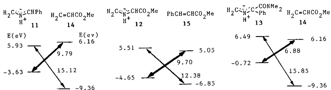
Fig. 1 HOMO-LUMO Correlation Diagram in 1,3-Dipolar Cycloaddition
