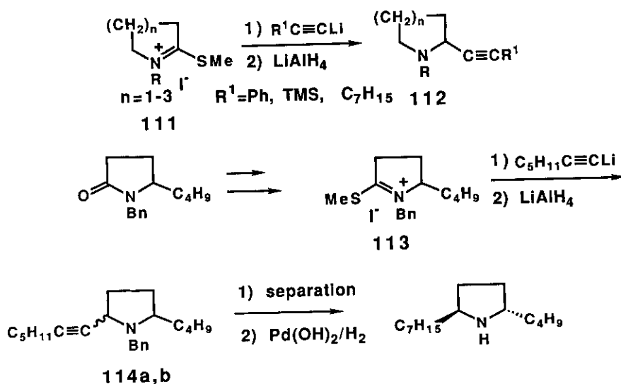
Scheme 22
