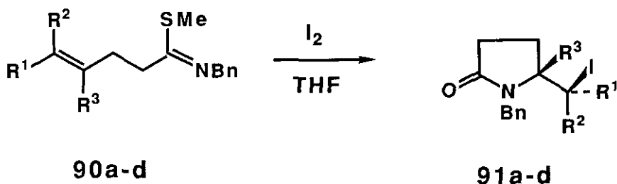
Scheme 17
