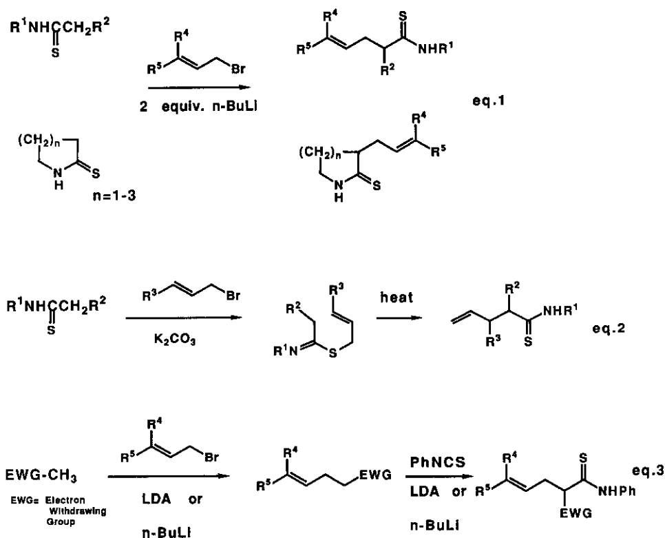
Scheme 15
