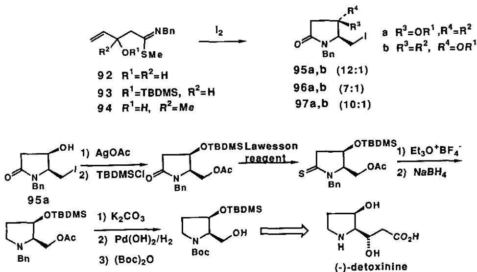
Scheme 18
