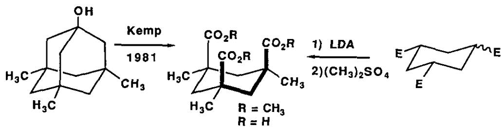
Synthesis of Kemp's triacid
