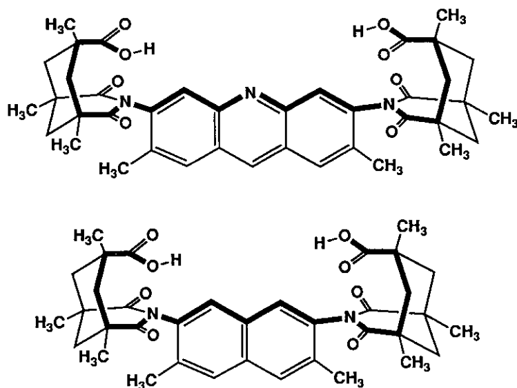
Molecular clefts derived from aromatic spacers
