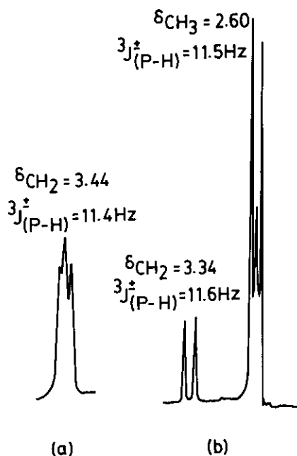
Figure 5. ^1\text{H} nmr spectra (100 MHz, \text{CDCl}_3 ) of (a) \text{N}_3\text{P}_3\text{Cl}_4(\text{NHCH}_2\text{CH}_2\text{NH}) (6) and b) \text{N}_3\text{P}_3(\text{NCH}_3)_4(\text{NHCH}_2\text{CH}_2\text{NH}) (6b) (NH regions not shown). From ref. 16
