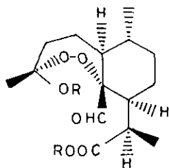
140 : R = Me
