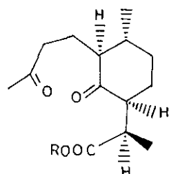
141 : R = Me
