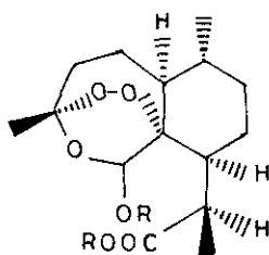
139 : R = Me
