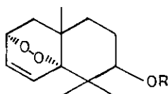
90 : R = PhCO
