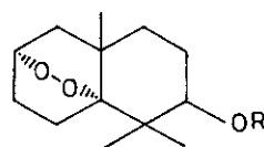
94 : R = PhCO
