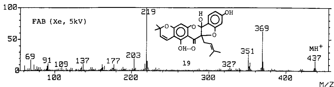
Figure 16 FAB mass spectrum of sanggenon A (19).
