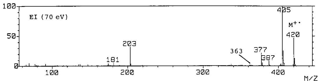
Figure 1 EI mass spectrum of morusin (1).
