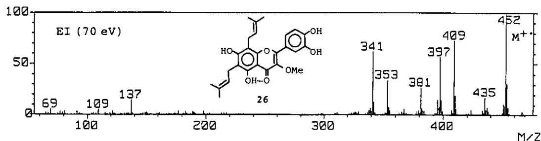
Figure 12 EI mass spectrum of brousoflavonol B (26).
