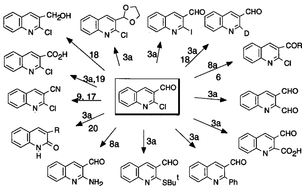
Functional group interconversions of 2-chloroquinoline-3-aldehyde
