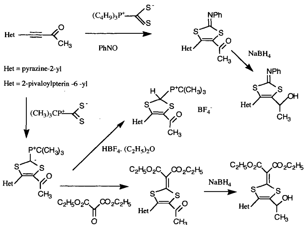
Scheme 5
