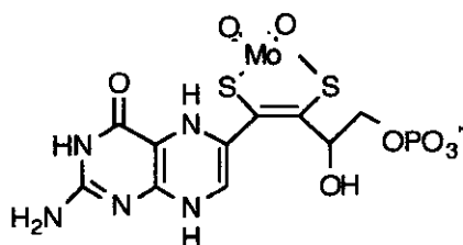
5,8-Dihydro
