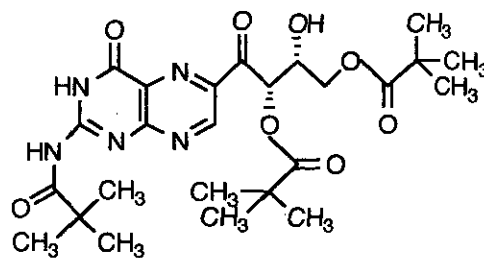
10 (or enantiomer)
