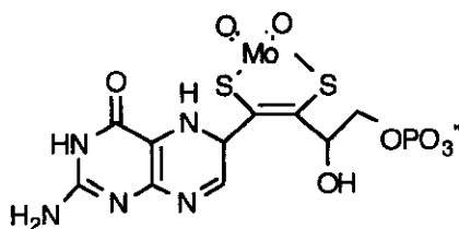
5,6-Dihydro
