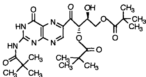
9 (or enantiomer)
