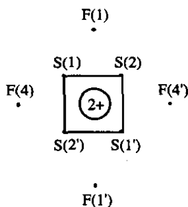
Figure 1 Structure of the \text{S}_4^{2+} cation in \text{S}_4(\text{AsF}_6)_2 \cdot 0.62\text{SO}_2 and nearest fluorine contacts from neighbouring \text{AsF}_6^- anions: \text{S}(1)-\text{S}(2) , 2.015(3); \text{S}(1)-\text{S}(2') , 2.013(3); \text{S}(1)-\text{F}(1) , 2.763(6); \text{S}(1)-\text{F}(4) , 2.736(7); \text{S}(2)-\text{F}(1) , 2.671; \text{S}(2)-\text{F}(4') , 2.664(6) Å; \angle \text{S}(2')\text{S}(1)\text{S}(2) , 90.5(1); \text{S}(1)\text{S}(2)\text{S}(1') , 89.5(1)°
