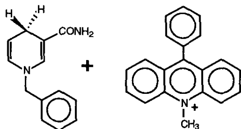
Linear Hydride Transfer (Verhoeven et al. )
