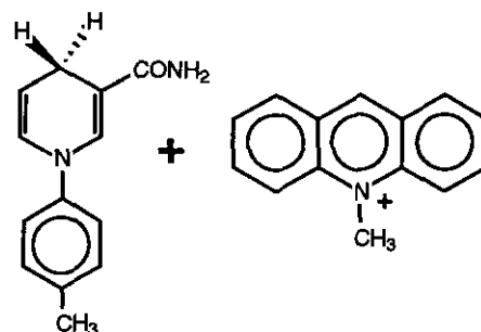
Bent Hydride Transfer with Tunnelling (Bruice et al. )
