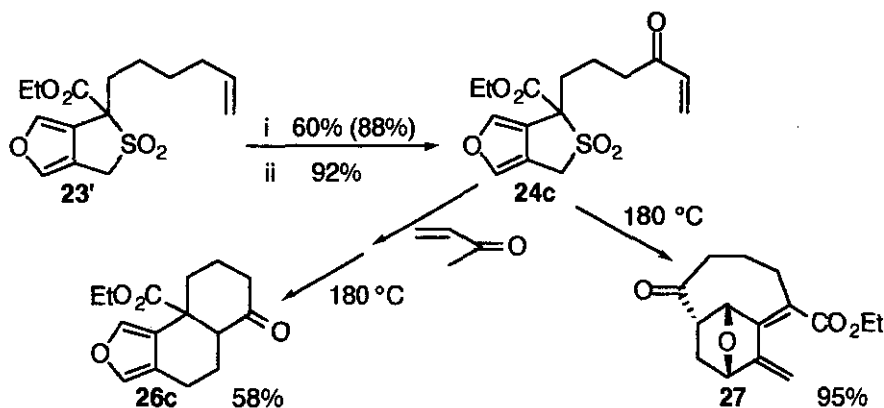
Scheme 6 Reagents and conditions : i, \text{SeO}_2 , t\text{-BuOOH} ; ii, \text{Me}_2\text{SO} , (\text{COCl})_2 , \text{Et}_3\text{N} ; (Yield based on consumed 23' in parentheses).
