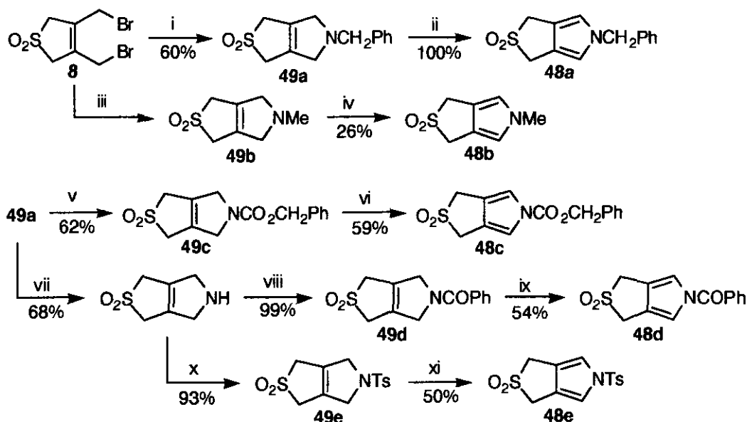
Scheme 9 Reagents and conditions : i, \text{PhCH}_2\text{NH}_2 , \text{MeCN} ; ii, DDQ, dioxane; iii, \text{MeNH}_2 , \text{MeCN} ; iv, DDQ, \text{C}_6\text{H}_6 ; v, \text{ClCO}_2\text{CH}_2\text{Ph} , \text{C}_6\text{H}_6 ; vi, chemical manganese dioxide, \text{C}_6\text{H}_6 ; vii, \text{ClCO}_2\text{CHClMe} in \text{ClCH}_2\text{CH}_2\text{Cl} , then \text{MeOH} , 50^\circ\text{C} ; viii, \text{PhCOCl} , \text{K}_2\text{CO}_3 , \text{CHCl}_3 ; ix, p\text{-MeC}_6\text{H}_4\text{SO}_2\text{Cl} , pyridine.
