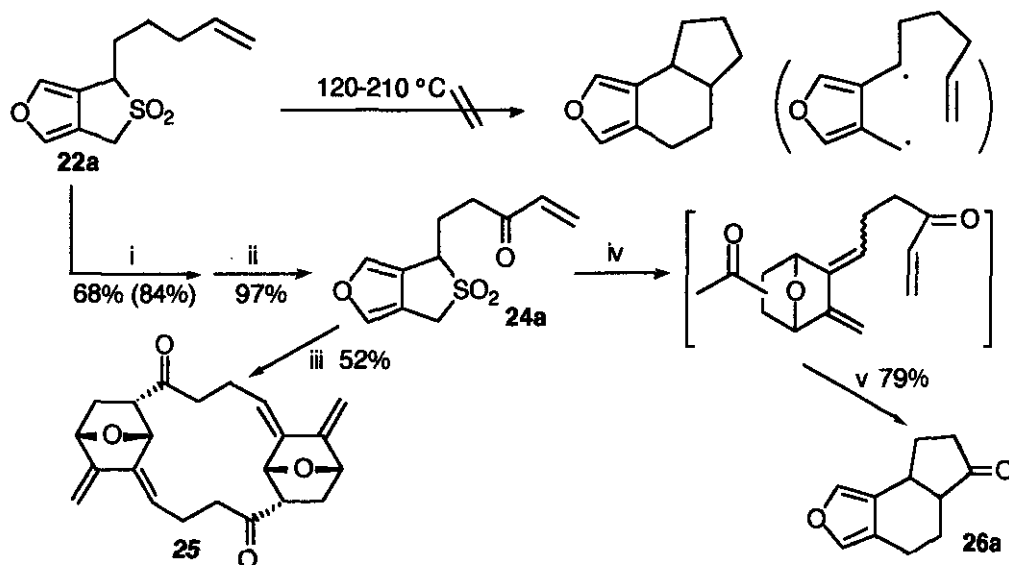
Scheme 4 Reagents and conditions : i, \text{SeO}_2 , t\text{-BuOOH} ; ii, \text{Me}_2\text{SO} , (\text{COCl})_2 , \text{Et}_3\text{N} ; iii, 120^{\circ}\text{C} , benzene; iv, methyl vinyl ketone, 25^{\circ}\text{C} ; v, 180^{\circ}\text{C} , toluene; (Yield based on consumed 22a in parentheses).
