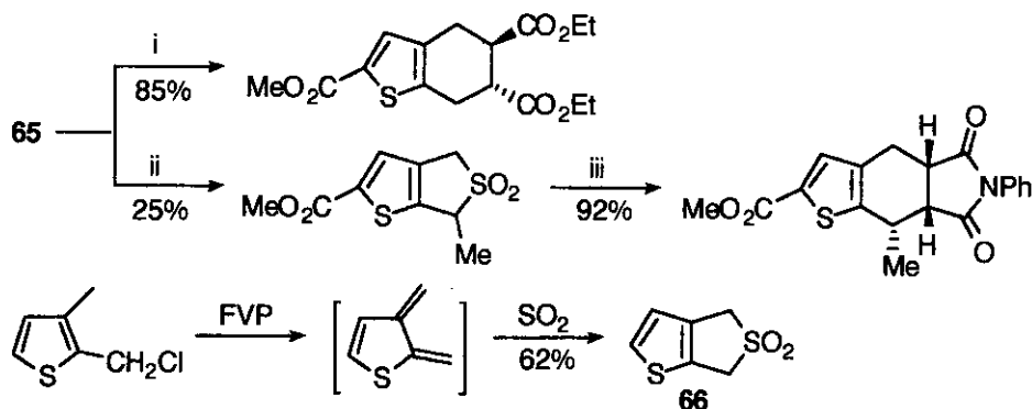
Scheme 14 Reagents and conditions : i, diethyl fumarate, sulfolane, 200 °C; ii, LDA, MeI, THF, -75 °C; iii, N-phenylmaleimide, sulfolane, 200 °C.
