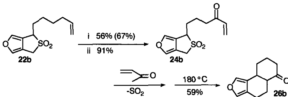
Scheme 5 Reagents and conditions : i, \text{SeO}_2 , t\text{-BuOOH} ; ii, \text{Me}_2\text{SO} , (\text{COCl})_2 , \text{Et}_3\text{N} ; (Yield based on consumed 22b in parentheses).
