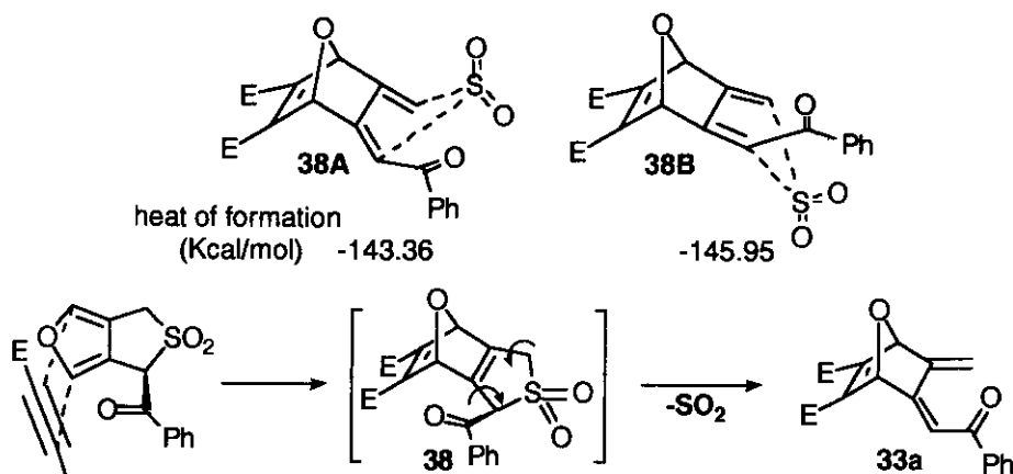
Scheme 7 Reaction mechanism
