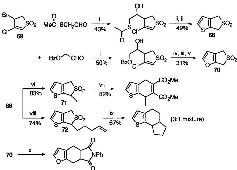
Scheme 15 Reagents and conditions : i, Zn, ultrasound, BF 3 ·Et 2 O; ii, KCN, NaHCO 3 ; iii, MeSO 2 Cl, Et 3 N, CH 2 Cl 2 ; iv, KCN, MeOH; v, NaOH, MeOH; vi, BuLi, -105 °C then MeI, -78 °C; vii, DMAD, 200 °C; viii, BuLi, HMPA then pent-4-enyl iodide; ix, 200 °C; x, N -phenylmaleimide, 160 °C, 3 h.
