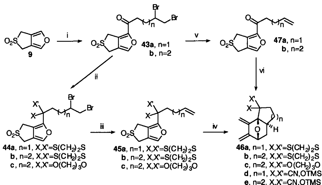
Scheme 8 Reagents and conditions : i, 4,5-dibromopentanoyl chloride or 5,6-dibromohexanoyl chloride, AlCl_3 in CH_2Cl_2 , 25 °C.; ii, 1,2-ethanedithiol or 1,3-propanediol / p -TsOH, reflux in benzene, 24 h; iii, Zn in THF-phosphate buffer, 25 °C, 1 h; iv, reflux in xylene, 2 h; v, TMSCN, KCN, 18-crown-6, reflux in benzene, 24 h.
