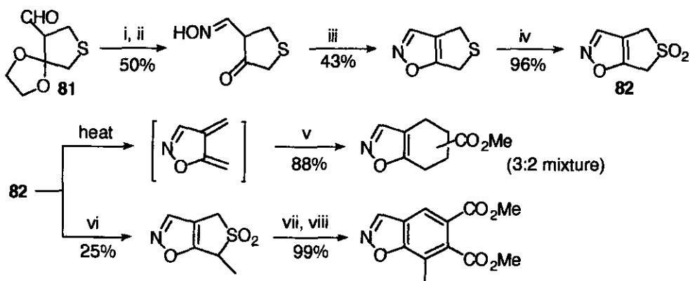
Scheme 20 Reagents and conditions : i, 20% \text{H}_2\text{SO}_4 , 25 °C; ii, \text{NH}_2\text{OH}\cdot\text{HCl} ; iii, polyphosphoric acid; iv, m CPBA, \text{CH}_2\text{Cl}_2 ; v, methyl acrylate, 160 °C, \text{CHCl}_3 ; vi, LiHMDS, HMPA, THF, then MeI (5 eq.), -78 °C; vii, DMAD (1.2 eq.), toluene, 180 °C; viii, DDQ, 140 °C.
