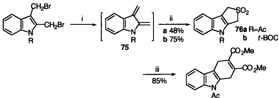
Scheme 17 Reagents and conditions : i, \text{NaI} , acetone, -30^\circ\text{C} ; ii, \text{SO}_2 ; iii, \text{DMAD} , 80\text{--}110^\circ\text{C} .
