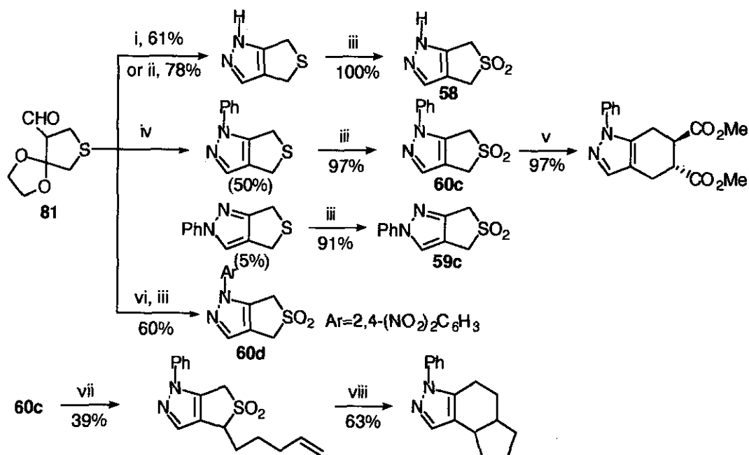
Scheme 21 Reagents and conditions : i, hydrazine hydrate (10 eq.), dioxane-5% HCl (3:1) then 10% \text{H}_2\text{SO}_4 ; ii, t BocNHNH 2 (1.1 eq.), TsOH, THF then 20% \text{H}_2\text{SO}_4 ; iii, m CPBA; iv, PhNHNH 2 (1.1 eq.), TsOH, THF then 30% \text{H}_2\text{SO}_4 -THF (1:1); v, dimethyl fumarate, 180 °C; vi, 2,4-dinitrophenylhydrazine, TsOH, THF then conc. \text{H}_2\text{SO}_4 - 95% EtOH (1:5); vii, LiHMDS (1.2 eq.), HMPA then 5-bromo-1-pentene, -105 °C; viii, toluene, 180 °C.
