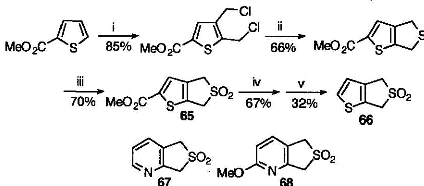
Scheme 13 Reagents and conditions : i, \text{ClCH}_2\text{OCH}_3 , \text{ZnCl}_2 ; ii, \text{Na}_2\text{S} , MeOH; iii, \text{H}_2\text{O}_2 , AcOH; iv, KOH, \text{H}_2\text{O} then \text{Br}_2 ; v, Pd/C, MeOH.
