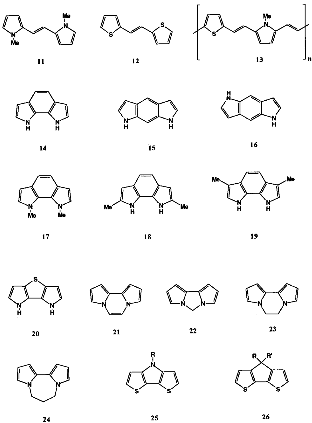
Scheme 5
