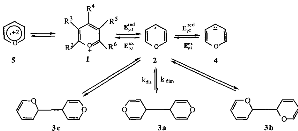
Scheme 1. One-electron transfer reactions of pyrylium heterocycles.
