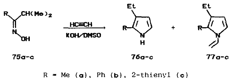
Scheme 31
