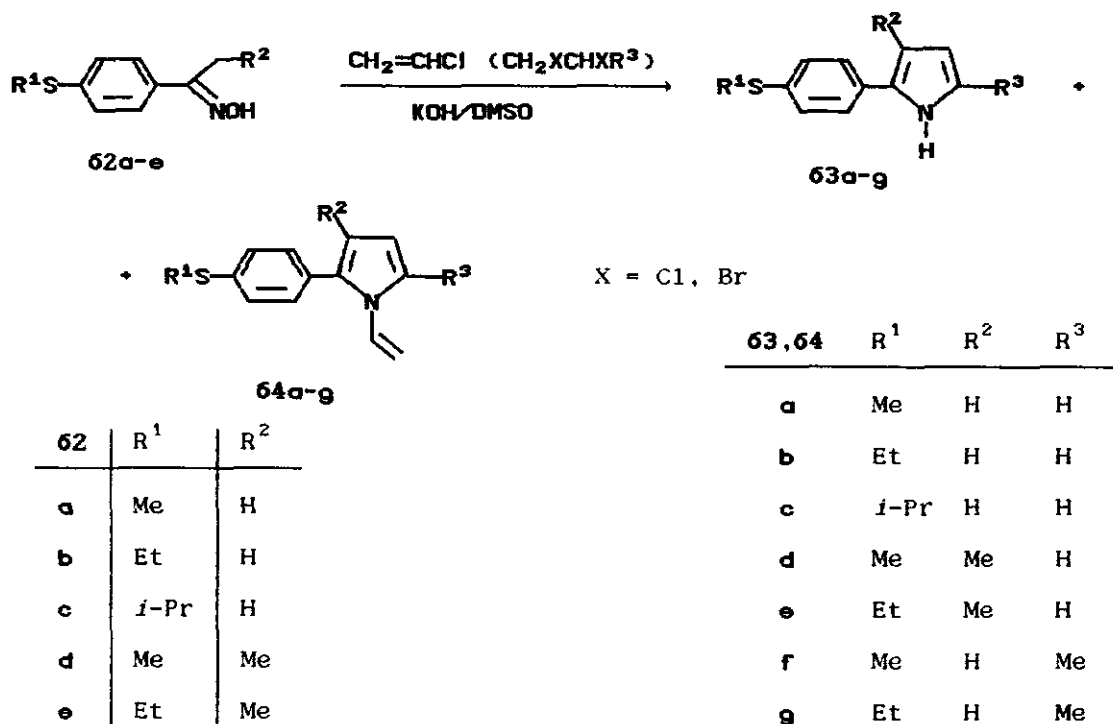
Scheme 25
