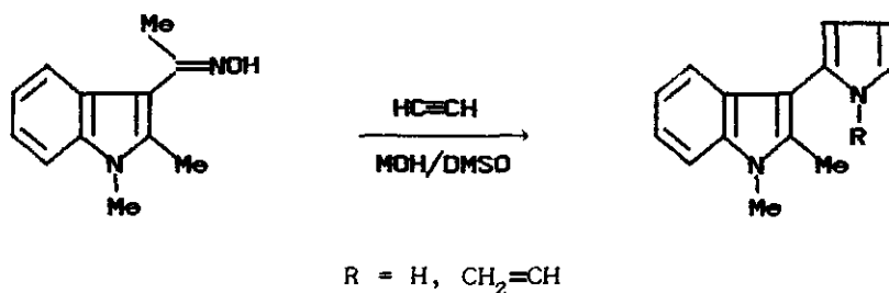
Scheme 16
