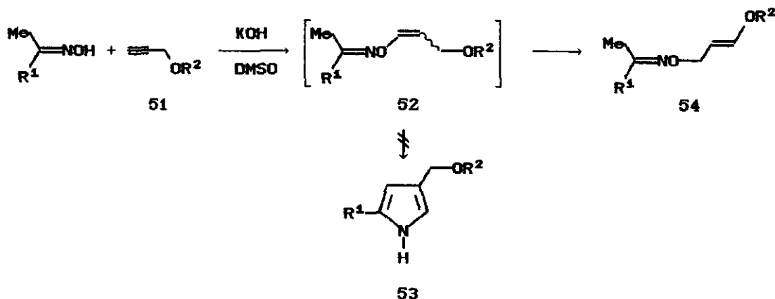
Scheme 21
