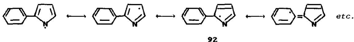
Scheme 37
