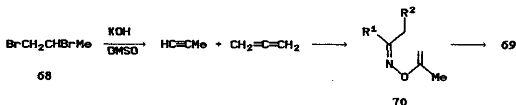
Scheme 28
