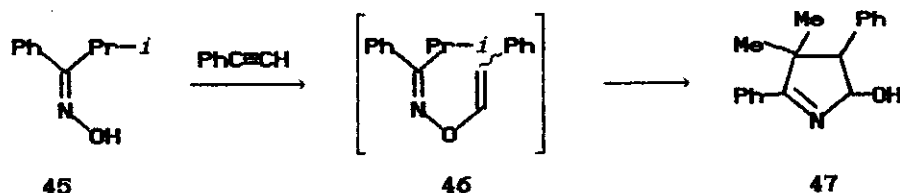
Scheme 19
