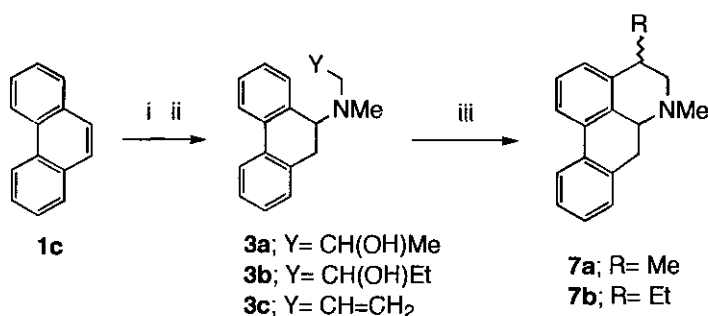
Scheme 4. Reagents: i h\nu / \text{H}_2\text{NCH}_2\text{-Y} / p -DCB, ii \text{HCO}_2\text{H/HCHO} , iii \text{CF}_3\text{SO}_3\text{H}
