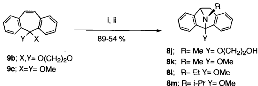
Scheme 7. Reagents; i h\nu /RNH 2 / p -DCB, ii AcOH
