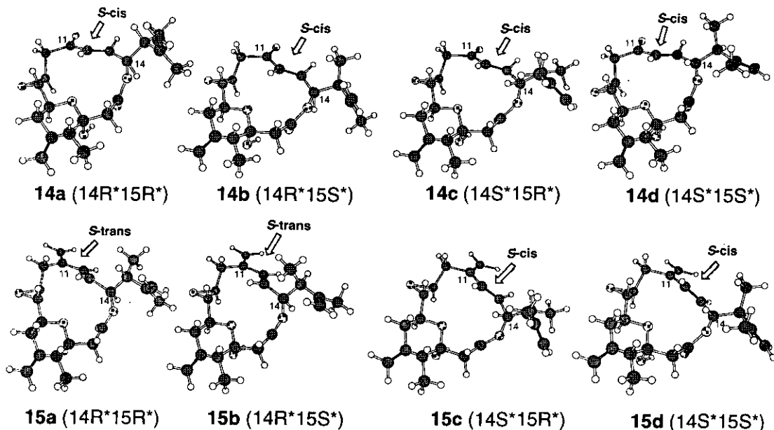
Figure 1. Three-Dimensional Structures of the Lowest-Energy Conformers of the Diastereomers ( 14a - 14d ) and ( 15a - 15d )
