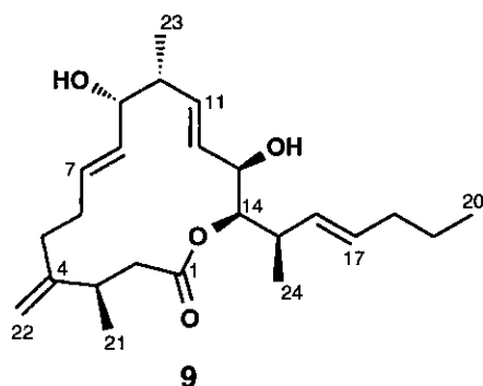
Figure 10. Labeling patterns of amphidinolide J ( 9 )
