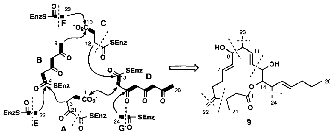
Figure 11. Possible Biosynthetic Building Blocks of Amphidinolide J ( 9 )
