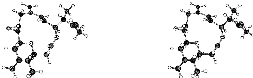
Figure 3. Stereoview of the Monte Carlo lowest-energy conformation of 15
