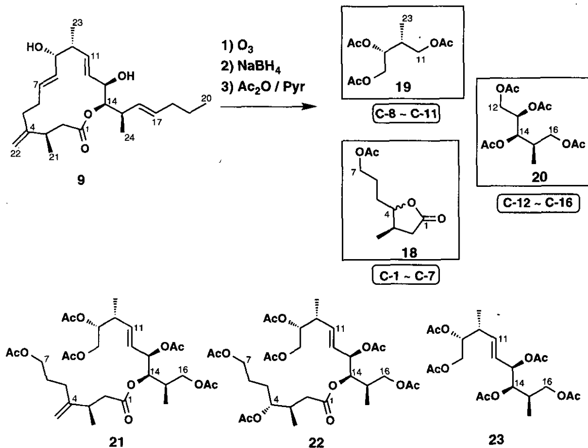
Scheme 1. Ozonolysis of Amphidinolide J ( 9 )
