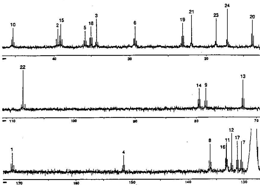
Figure 9. The ^{13}\text{C} Nmr spectrum of 9 labeled with sodium [1,2-^{13}\text{C}_2] acetate
