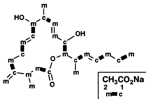
Figure 10. Labeling patterns of amphidinolide J ( 9 )
