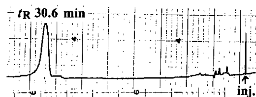
Figure 5. Hplc Comparison of Amphidinolide B and Amphidinolide B 1
