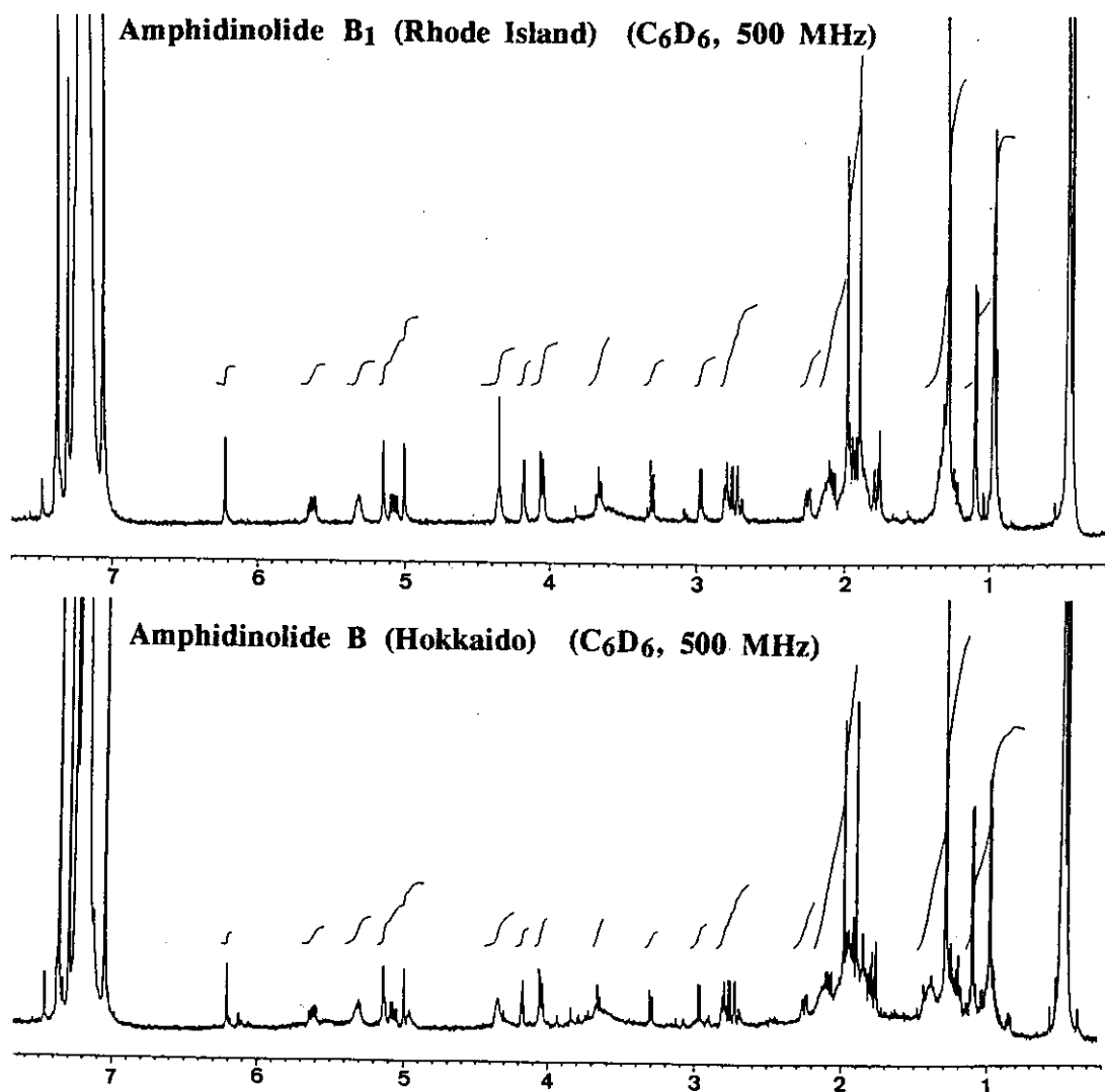
Figure 6. ^1\text{H} Nmr Comparison of Amphidinolide B and Amphidinolide B 1
