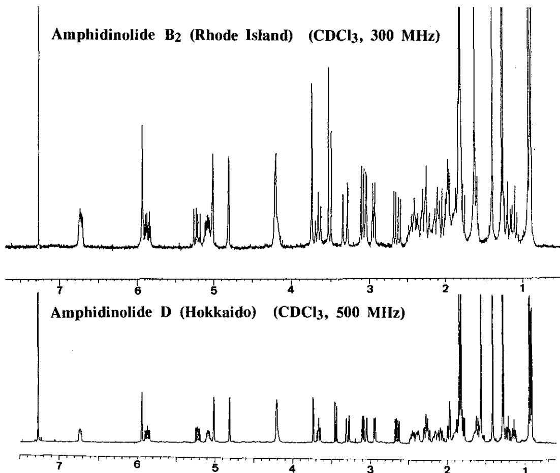
Figure 7. ^1\text{H} Nmr Comparison of Amphidinolide D and Amphidinolide B 2
