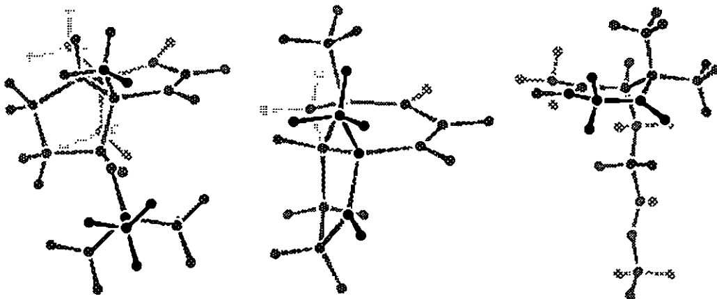
Figure 2 : Lowest energy conformers of 32 , 34 and 39 used to predict face selectivity.
