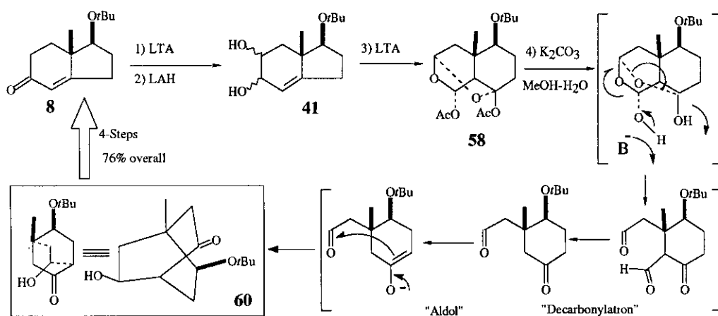
Scheme 16: The bicyclo[2.2.2]octane framework via two consecutive cascade transformations.
