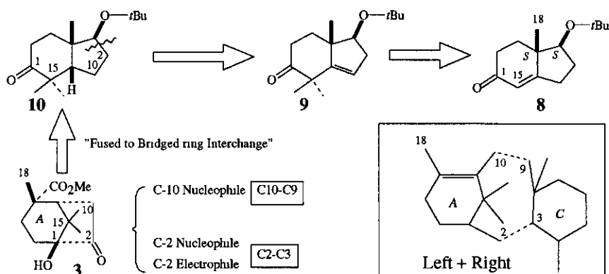
Scheme 3 : Retrosynthetic analysis for the left-half building unit ( 3 ).
