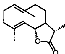
(125)
