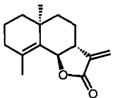
(78)
