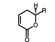
(312) R=-(CH 2 ) 6 Me
