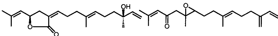
(277)
