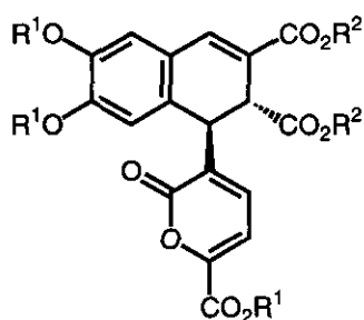
(392) R^1=R^2=R^3=H
