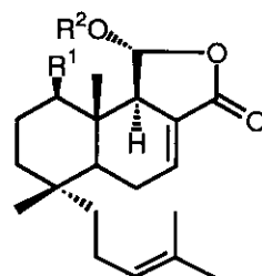
(284) R^1=R^2=H
