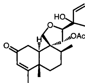
(219)
