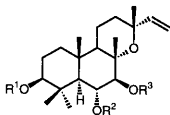
(273) R^1=R^2=Ac , R^3=H
