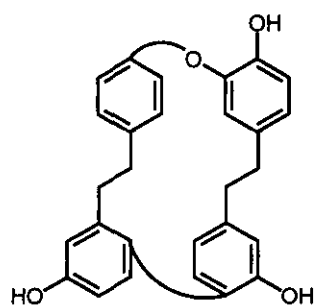
(351)
