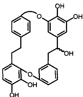
(361)
