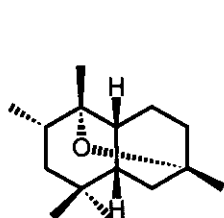
(185)
