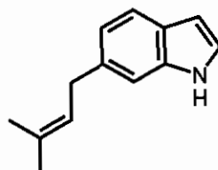
(433)
