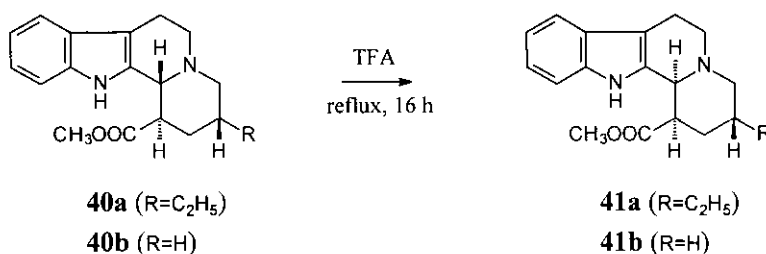
Scheme 15
