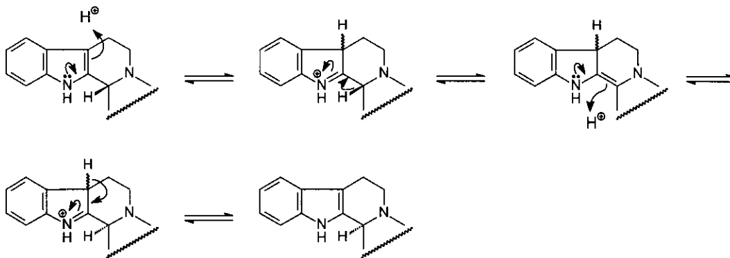
Scheme 1 (Mechanism 1)
