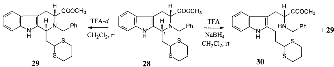
Scheme 10
