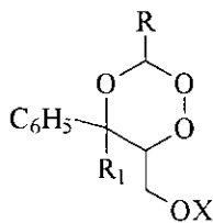
157 b R=R_1=\text{C}_2\text{H}_5 , X=\text{CONHC}_6\text{H}_5 c R=\text{C}_3\text{H}_7 , R_1=\text{CH}_3 , X=\text{CONHC}_6\text{H}_5 d R=\text{C}_2\text{H}_5 , R_1=\text{CH}_3 , X=\text{COOCH}_3
