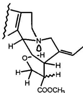
Figure 22. Compounds (17) and (18) in conformation c with ring D in twist-boat conformation.
