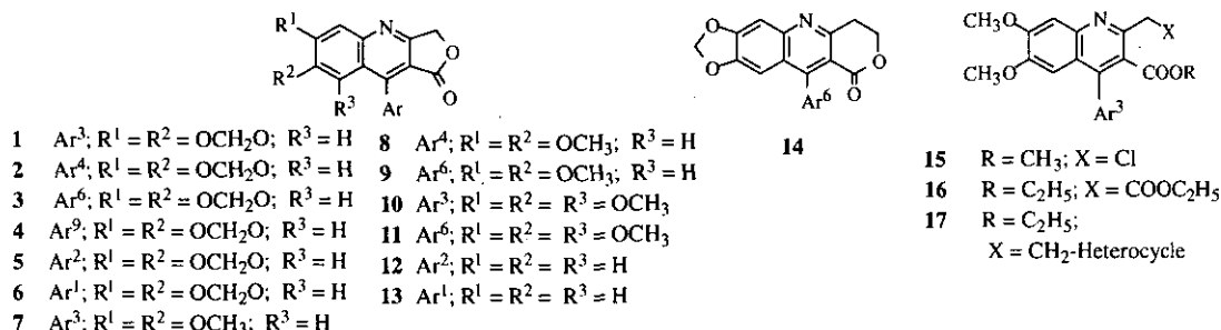
Figure 6. 7-Aza-heterolignans.
