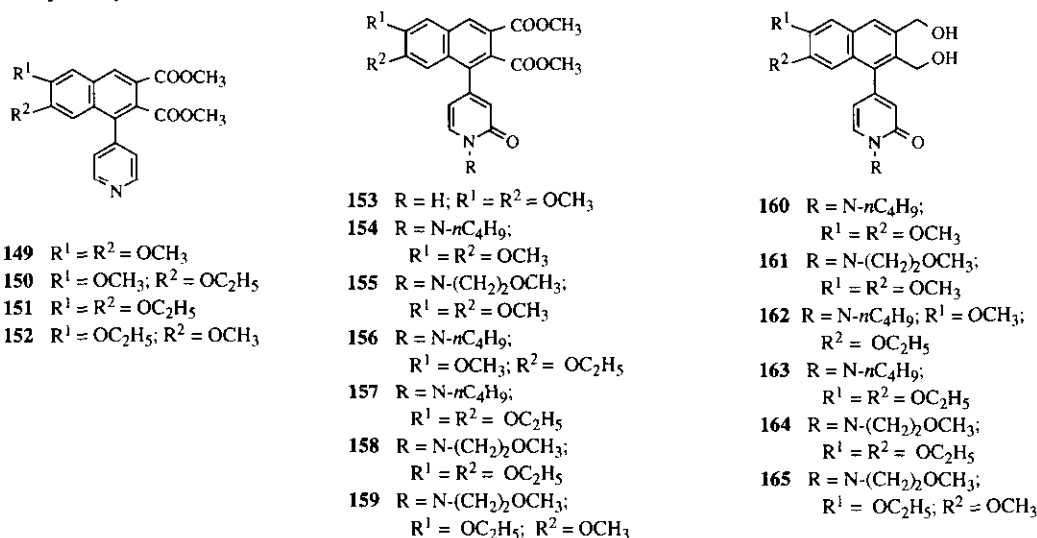
Figure 19. Naphthalenic heterolignans.
