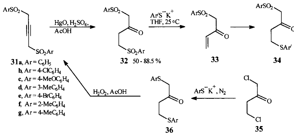
Scheme 7
