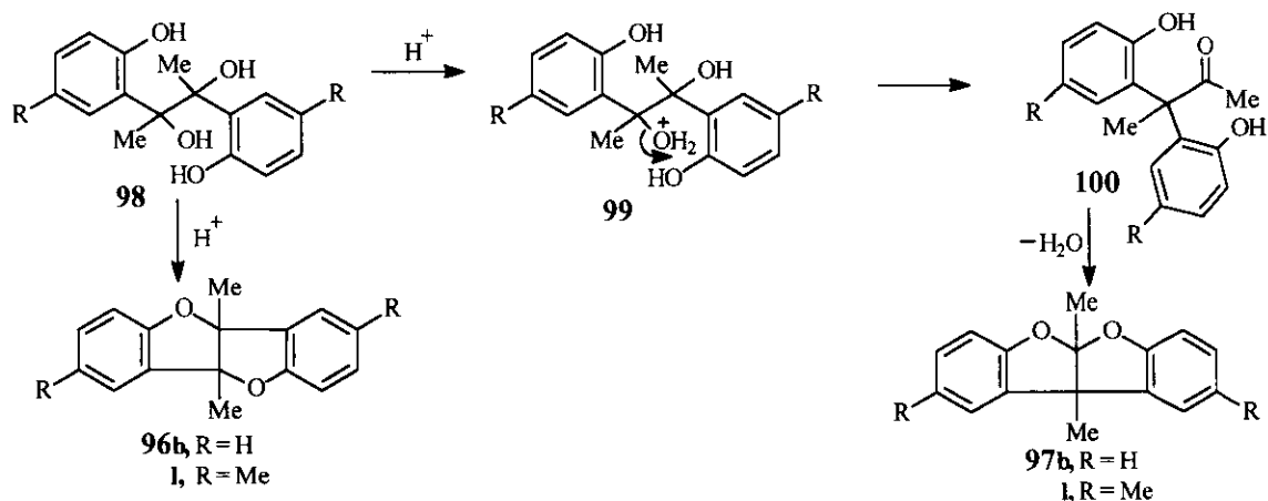
Scheme 26
