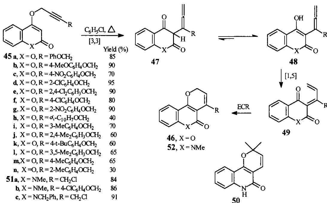
Scheme 11
