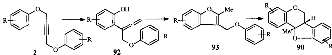
Scheme 21
