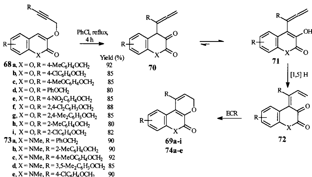
Scheme 15
