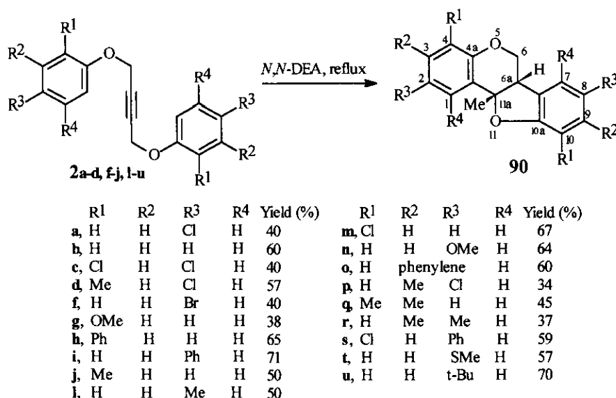
Scheme 19
