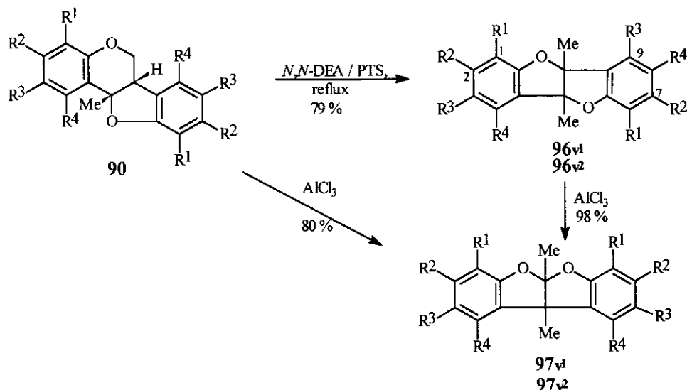
Scheme 32
