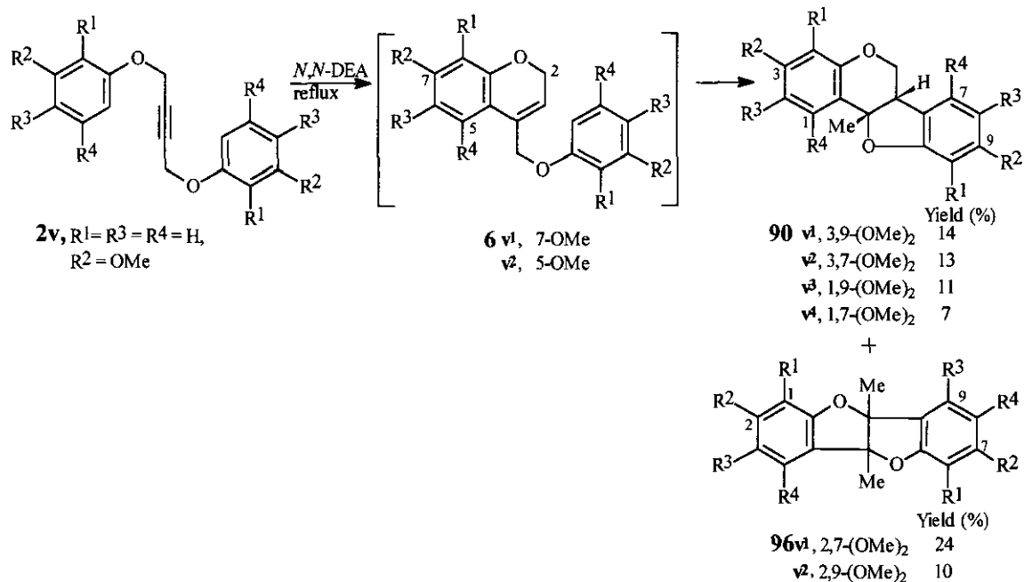
Scheme 23
