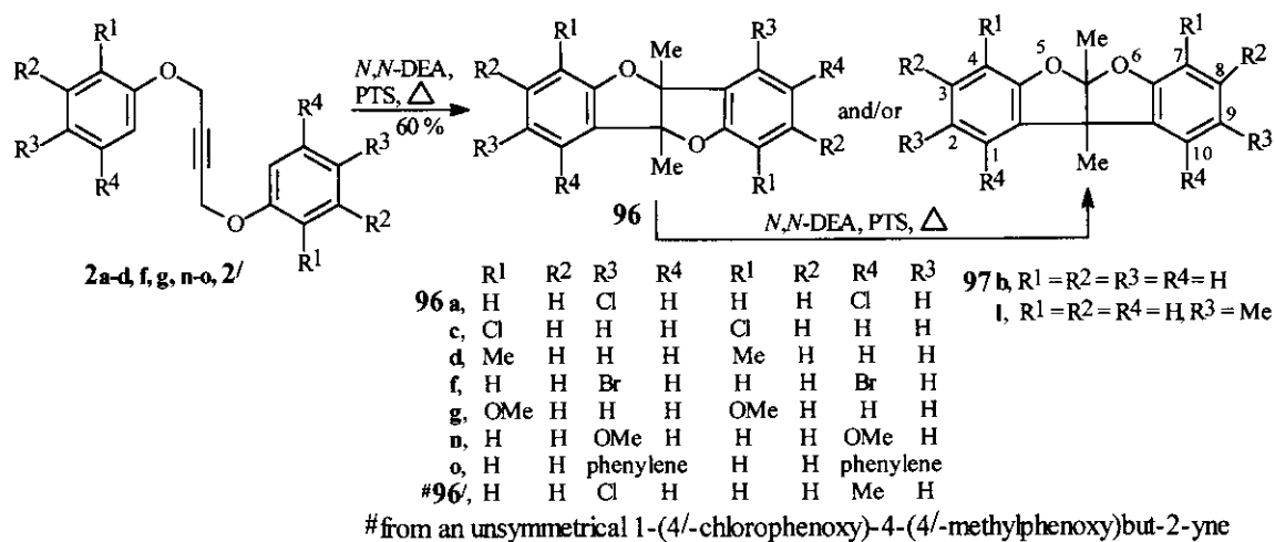
Scheme 25
