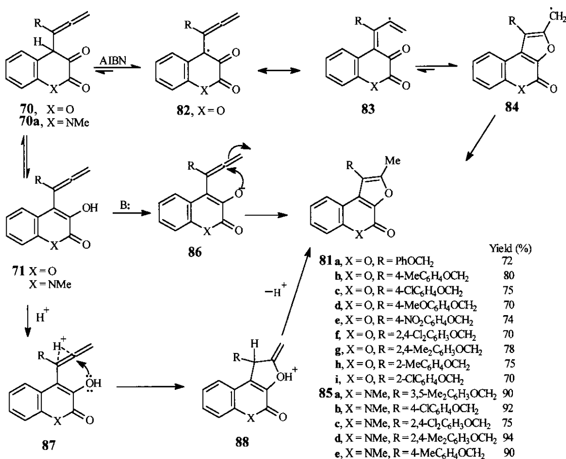
Scheme 17
