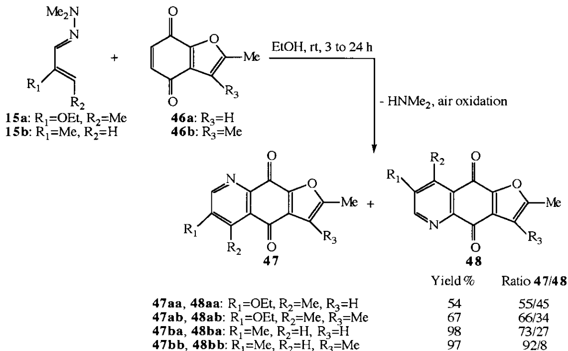
Scheme 25
