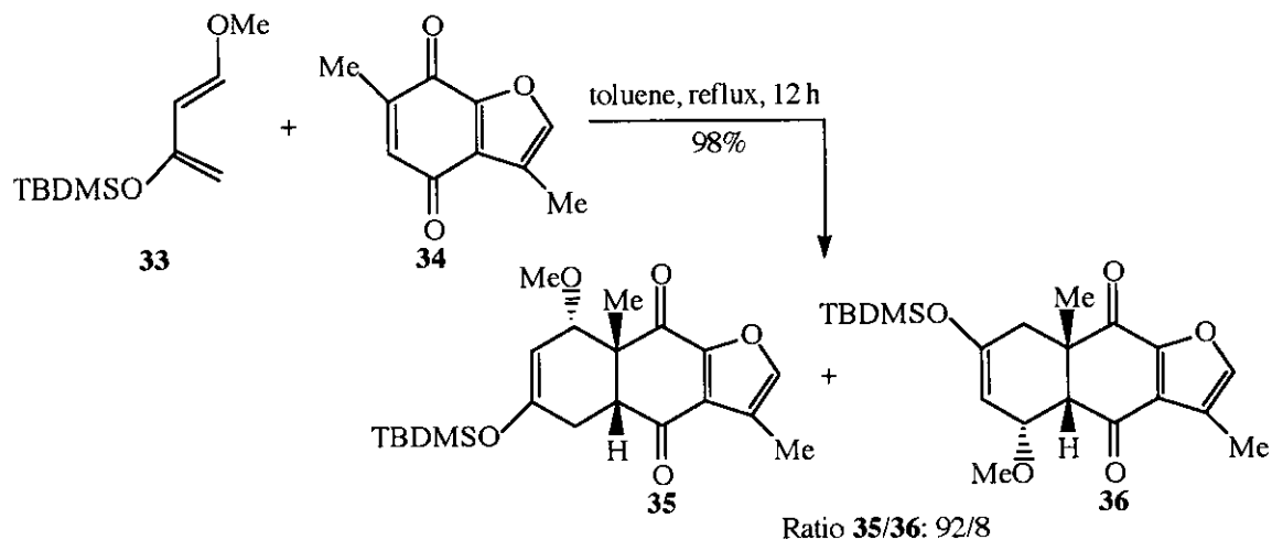
Scheme 19
