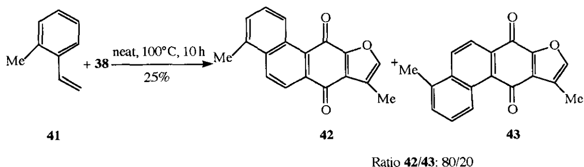
Scheme 23
