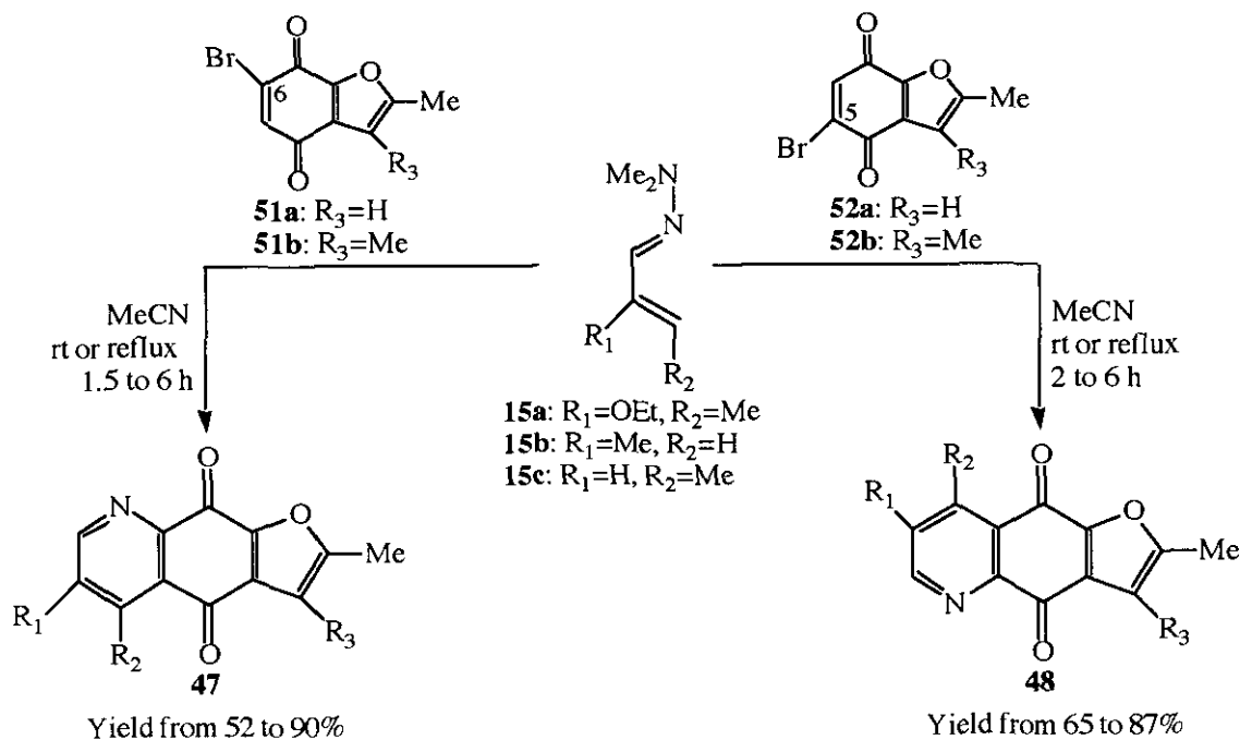
Scheme 27
