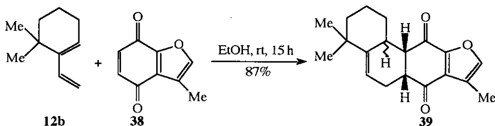
Scheme 21
