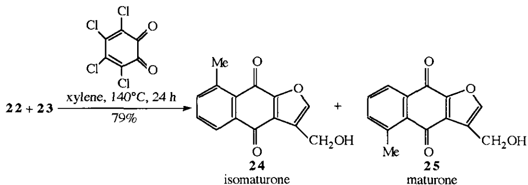
Scheme 14
