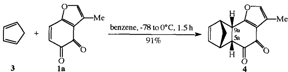
Scheme 6
