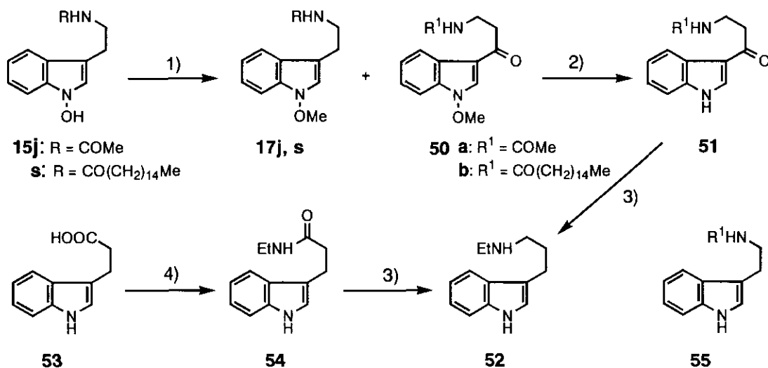
Scheme 7
