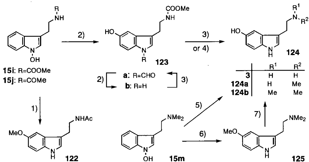
Scheme 13
