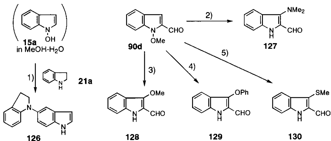
Scheme 14
