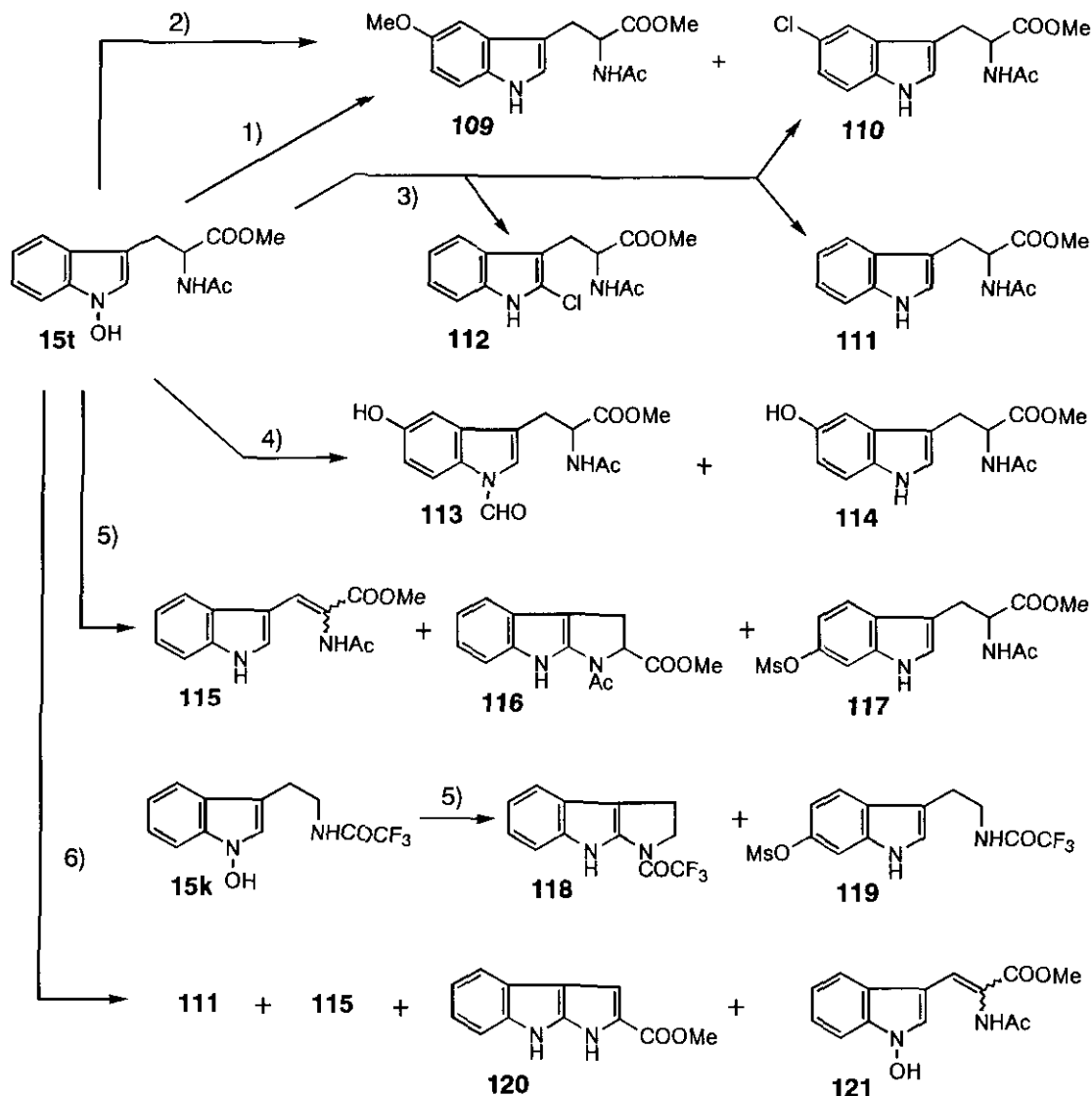
Scheme 12
