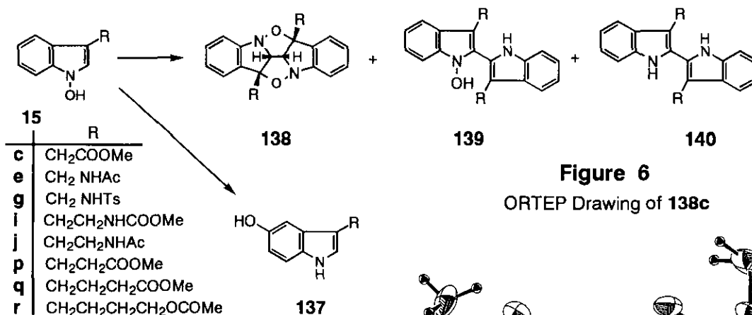
Scheme 15
