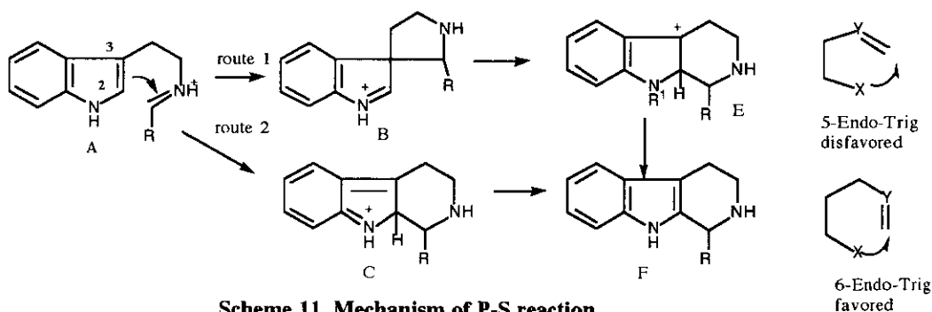
Scheme 11 Mechanism of P-S reaction
