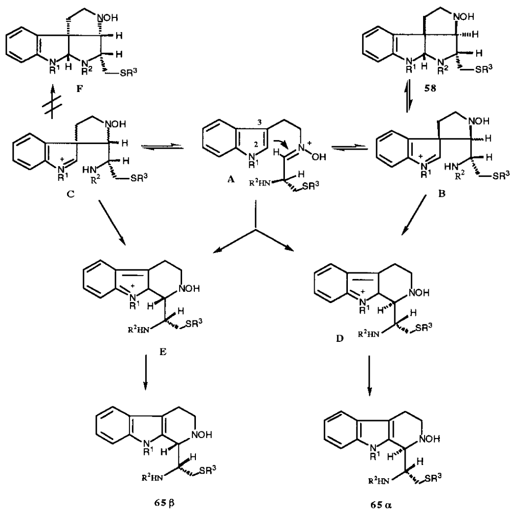
Schem 12 A proposed mechanism of cyclization of the nitron
