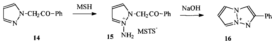
Scheme 8
