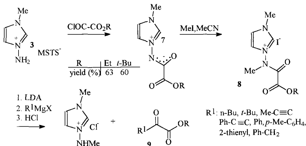
Scheme 5
