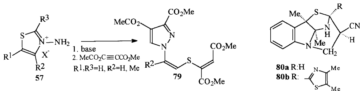
Scheme 27
