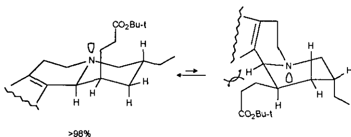
Scheme 30. Conformational equilibrium of compound (37).
