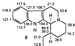
Figure 4. Measured 13 C NMR shift values of compound (6). 13
