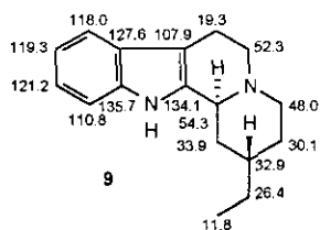
Figure 7. Measured ^{13}\text{C} NMR shift values of compound (9). 13
