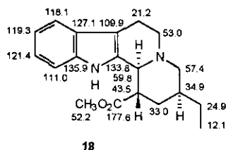
Figure 16. Measured ^{13}\text{C} NMR shift values of compound ( 18 ). 20
