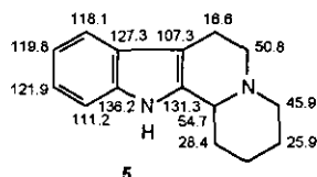
Figure 3. Estimated 13 C NMR shift values for conformation c of compound (5).
