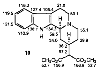
Figure 8. Measured 13 C NMR shift values of compound (10). 16
