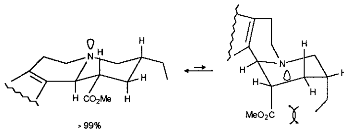
Scheme 16. Conformational equilibrium of compound (20).
