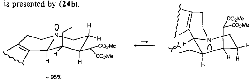
Scheme 21. Conformational equilibrium of compound (24b).
