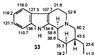
Figure 29. Measured ^{13}\text{C} NMR shift values of compound (33). 23
