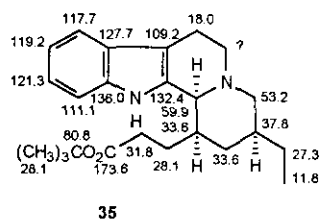
Figure 31. Measured ^{13}\text{C} NMR shift values of compound (35) (C-6 signal was not given). 29
