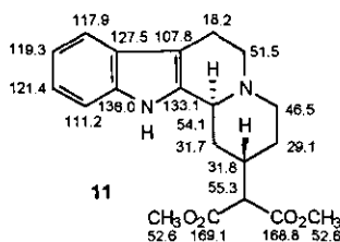
Figure 9. Measured 13 C NMR shift values of compound (11) (the original assignments given 16 for C-4 and C-6 are interchanged).
