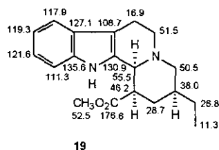
Figure 17. Measured ^{13}\text{C} NMR shift values of compound ( 19 ). 21
