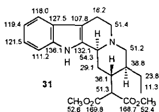
Figure 27. Measured ^{13}\text{C} NMR shift values of compound (31). 28
