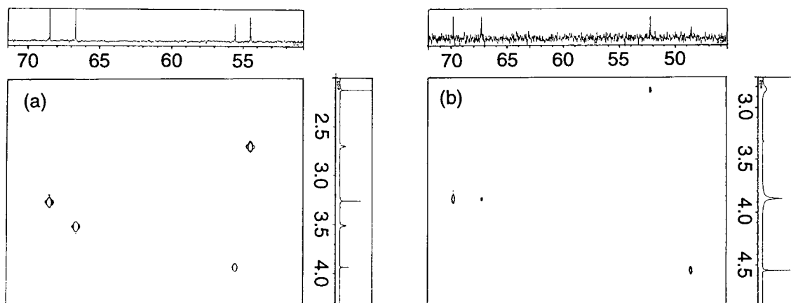
Figure 10. C-H COSY spectra of 2cN ( 1.0 \times 10^{-2} M) with (a) KSCN ( 1.0 \times 10^{-2} M) and (b) \text{Ba}(\text{SCN})_2 ( 1.0 \times 10^{-2} M) in \text{CDCl}_3\text{-CD}_3\text{CN} (1:1 v/v).
