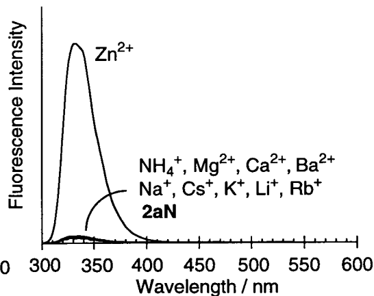
Figure 6. Fluorescence spectra of 2aN ( 2.00 \times 10^{-5} M) with and without various guest salts ( 5.00 \times 10^{-4} M) in methanol, as excited at 280 nm.
