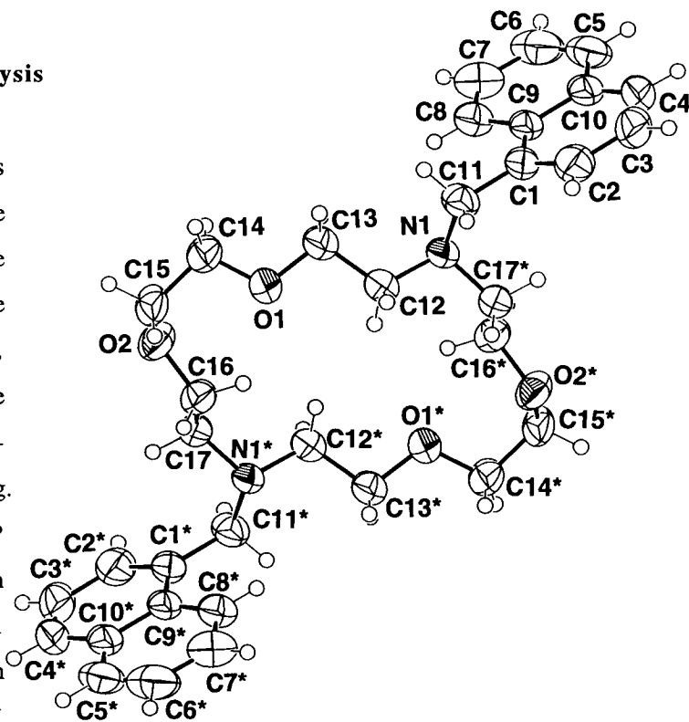
No \pi - \pi interaction is evident in the crystal packing; the distance between Figure 19. The molecular structure of 2cN with thermal ellipsoids to enclose 50% probability. Symmetry codes: (*) 1/2 - x, y, 1 - z
