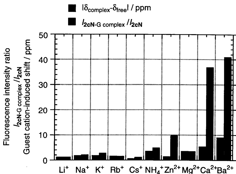
Figure 11. Guest cation-induced changes in ^{13}\text{C} NMR chemical shift of methylene carbon of naphthylmethyl group ( [2\text{cN}] = 1.0 \times 10^{-2} \text{ M} ) and in emission intensity ratio ( I_{2\text{cN-G complex}} / I_{2\text{cN}} , [2\text{cN}] = 2.0 \times 10^{-5} \text{ M} ); [\text{Guest cations}] = 1.0 \times 10^{-2} \text{ M} .
