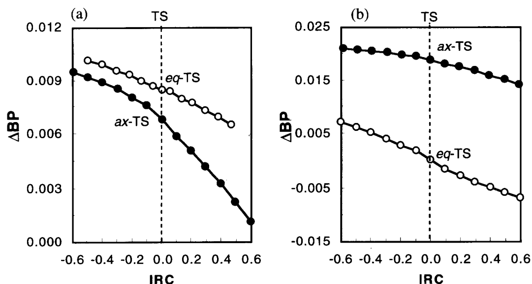
Figure 5 Plot of reduced bond population of the antiperiplanar bonds ( \Delta BP ) against the intrinsic reaction coordinate (IRC: unit; \text{amu}^{1/2} \text{ bohr} ) for the \text{LiAlH}_4 reduction of; (a) 1,3-dioxan-5-one ( 1b ) and (b) 1,3-dithian-5-one ( 2b ) (B3LYP/6-31+G(d) except for eq -TS of 1b for which B3LYP/6-31G(d) was used). (Filled circles; axial process; open circles; equatorial process)
