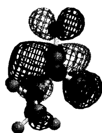
Cyclohexanone
