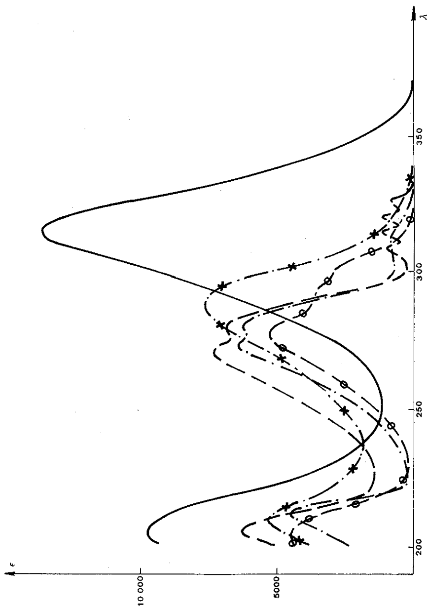
Fig. 3 uv spectra of (+)-VII in different solvents.
