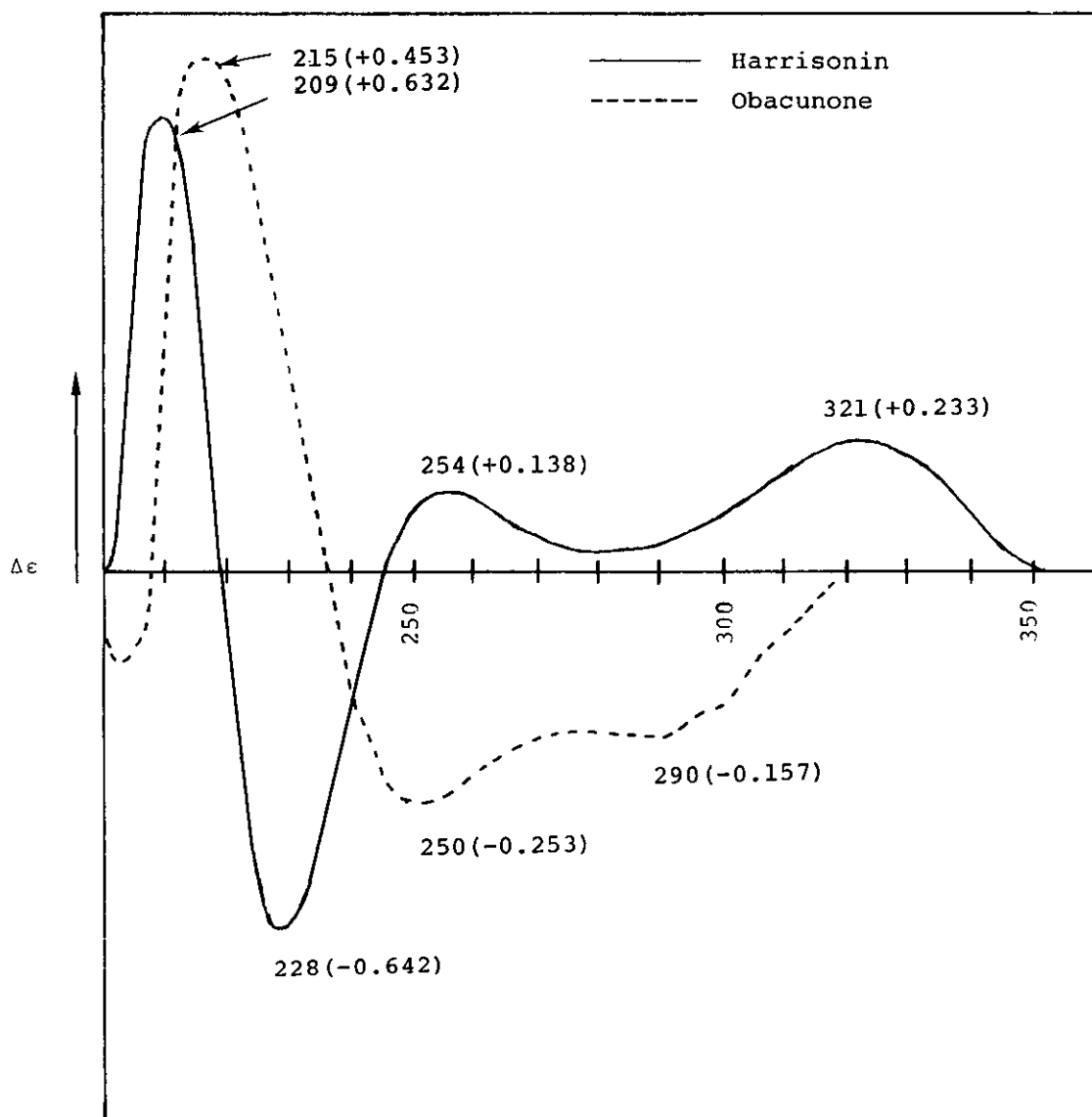
Fig.5 Cd spectra, nm( \Delta\epsilon ), in \text{CH}_3\text{OH}
