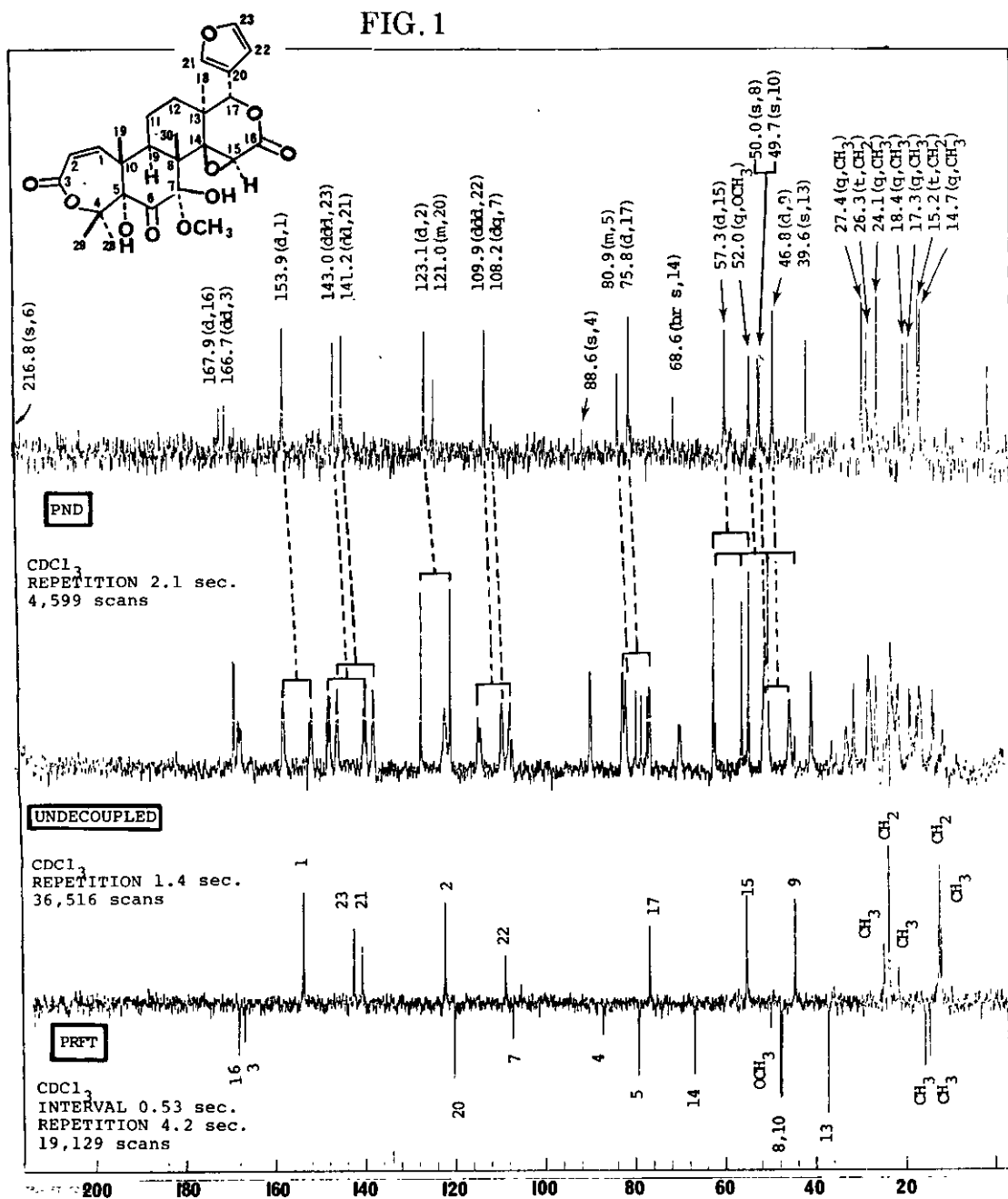
Fig.1 Cmr spectra of harrisonin, 25 MHz, \text{CDCl}_3
