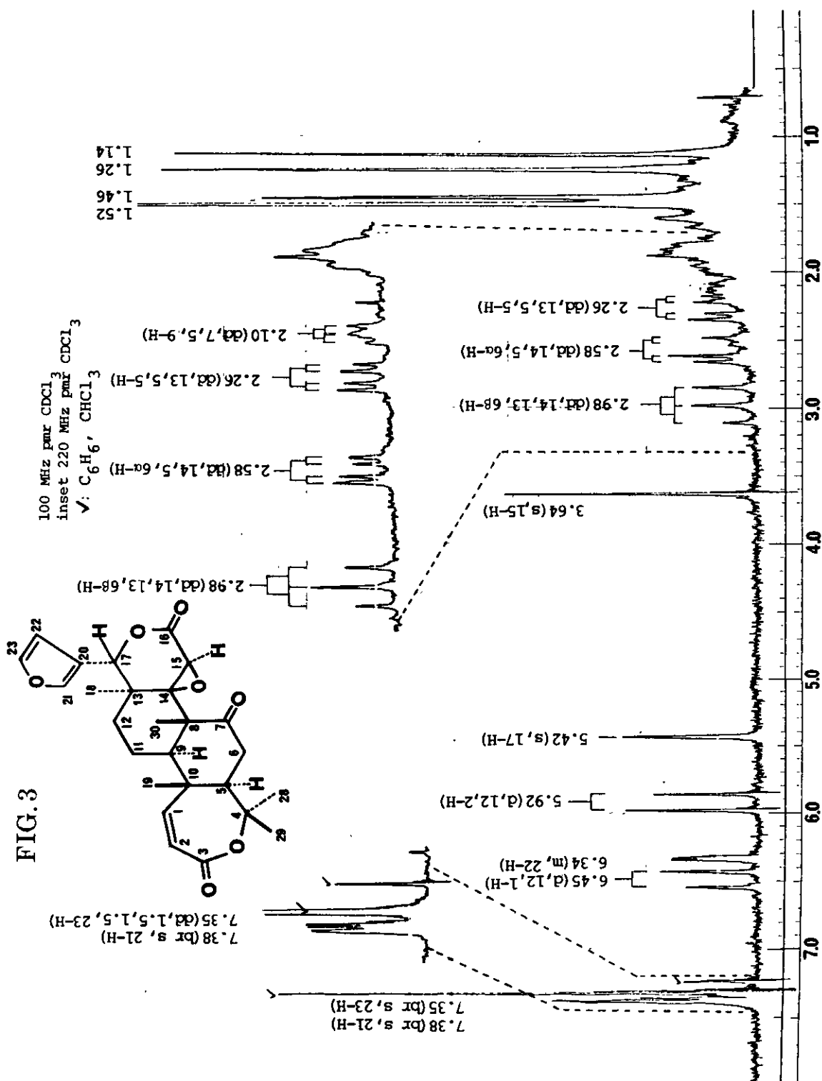
Fig. 3 Pmr spectra of obacunone, 100 MHz and 220 MHz (inset), \text{CDCl}_3
