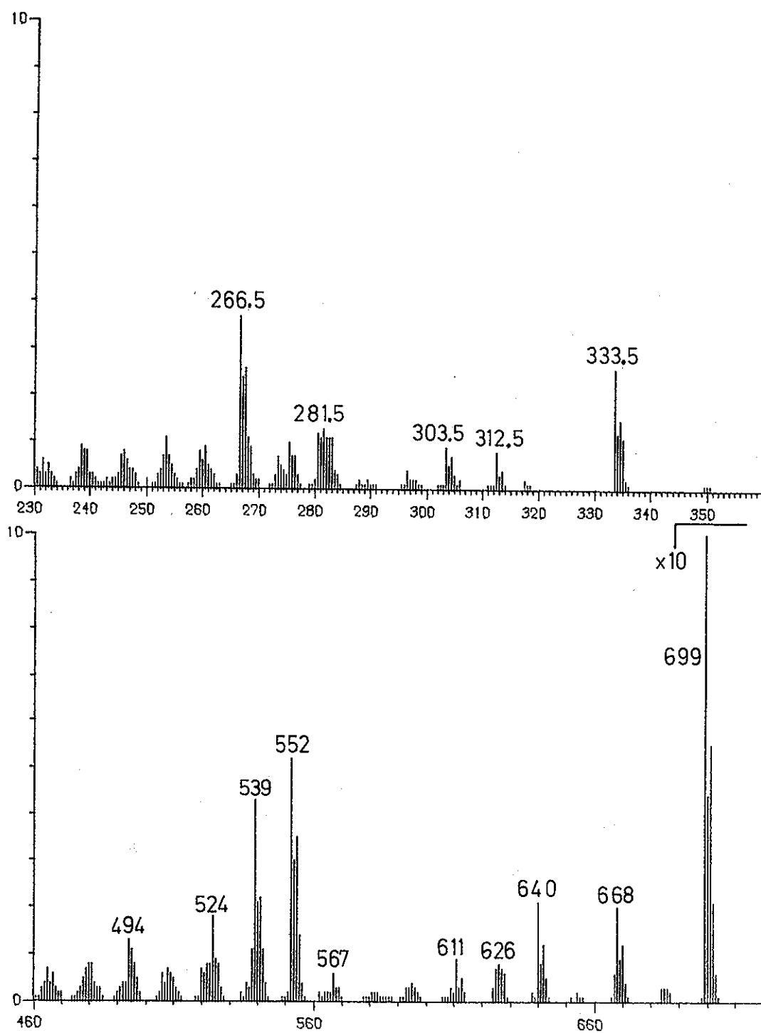
Fig.6 Mass spectrum of Cu chlorin e_6 trimethyl ester (Cu-4a) (MAT 731, 70 eV, probe 210^\circ , source 180^\circ ).
