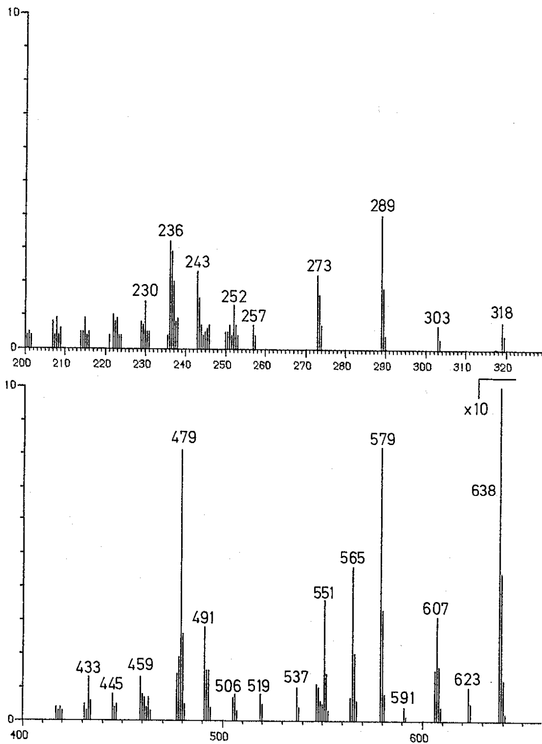
Fig.4 Mass spectrum of chlorin e_6 trimethyl ester (4a) (MAT 731, 70 eV, probe 200°, source 170°).
